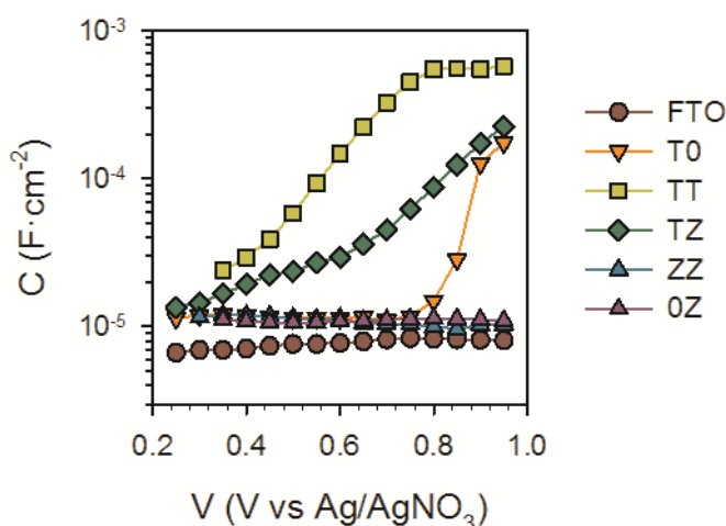
Figure 2: Capacitance of non-sensitized electrodes. Capacitance has been extracted from IS measurements in liquid electrolyte with I - /I 3- redox couple. Capacitance of bare conductive Sn 2 O:F (FTO) electrode is compared with electrodes with up to different layers of TiO 2 and ZrO 2 . The electrodes are called using the notation XY, where X is a compact layer and Y a porous layer, T and Z mean TiO 2 and ZrO 2 layer respectively. 0 means no layer i.e. T0 compact TiO 2 layer with no nanoporous layer.
