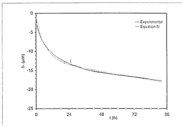
Fig. 14 Strain of a porcelain tile test piece under loading
