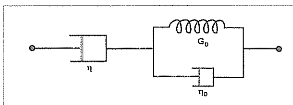
Fig. 15 Linear viscoelastic model used to model creep
