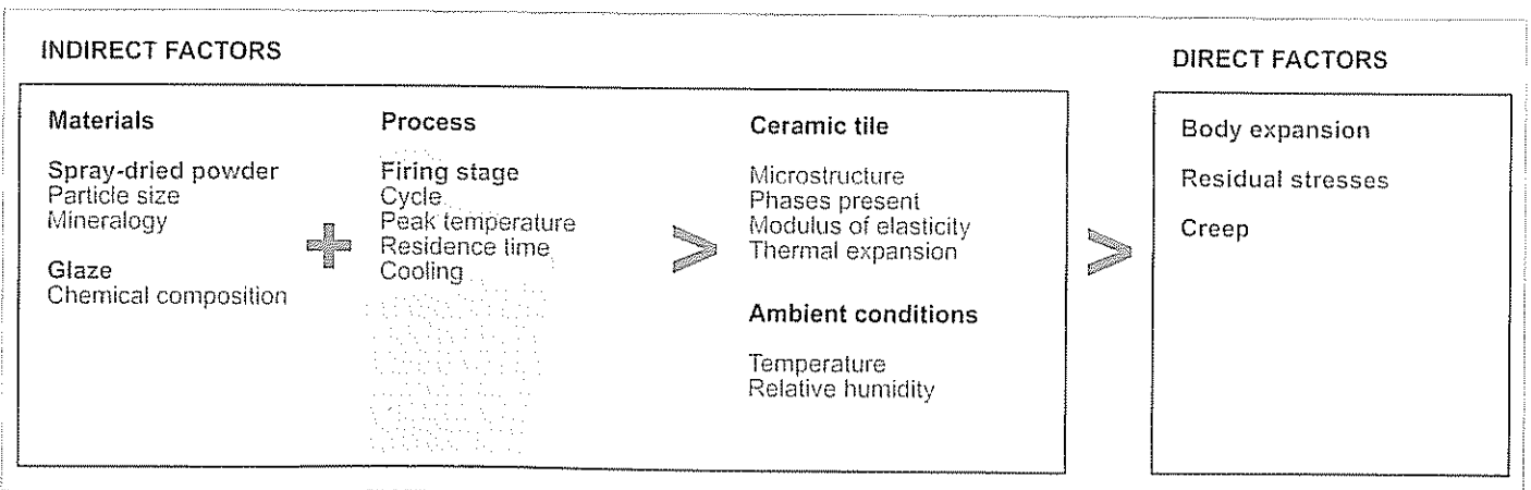
Fig. 16 Factors that influence delayed curvatures
