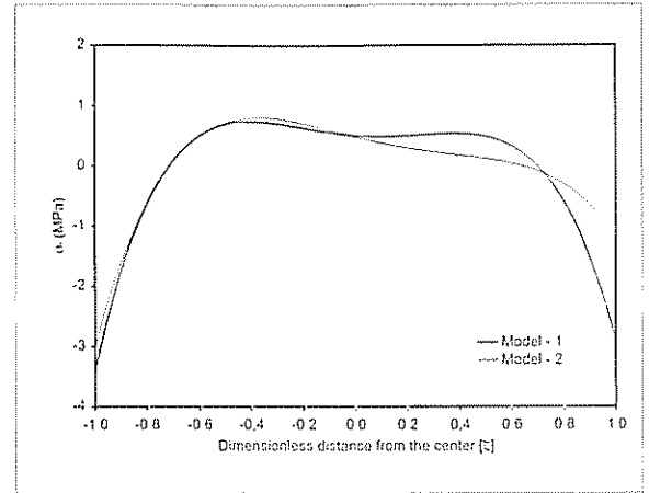
Fig. 12 Residual stress profiles of Model-1 and Model-2
