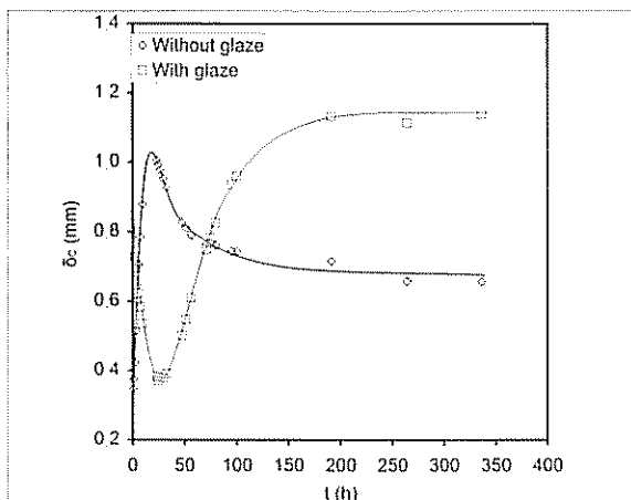
Fig. 19 Evolution of tile deflection with and without glaze
