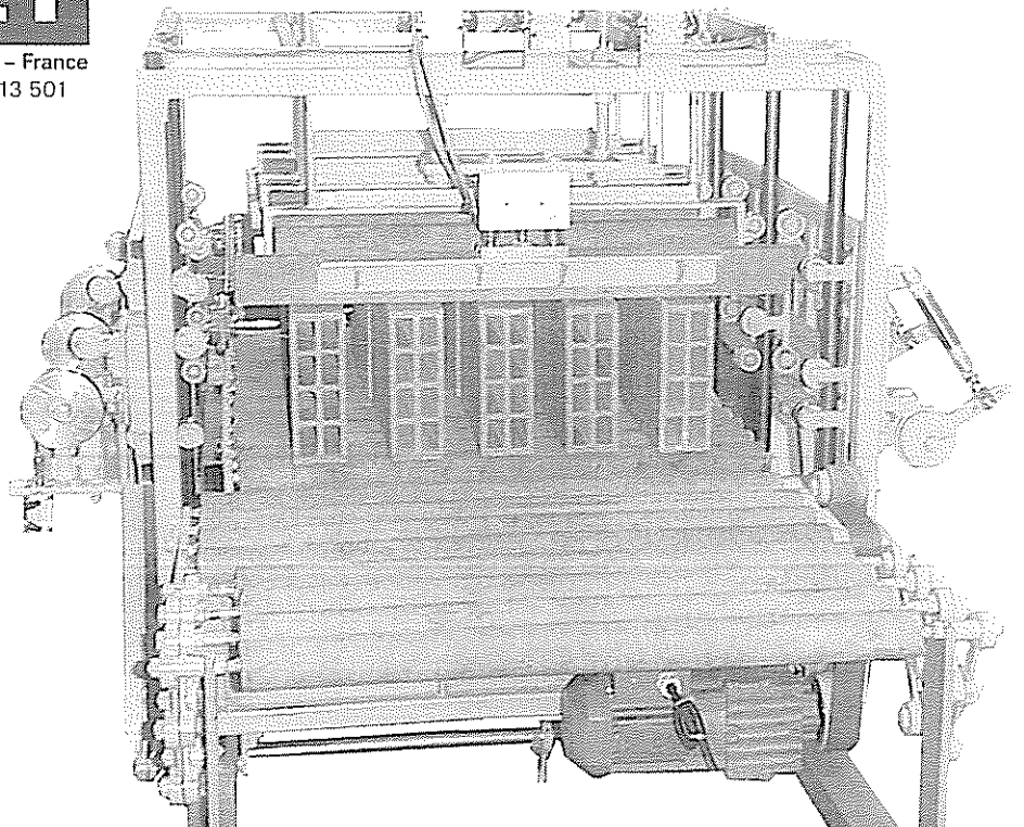
Five exits bricks cutter
