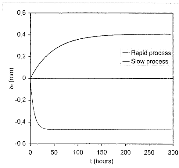
Fig 3 Contribution of both processes (Model 1, Tile 2)
