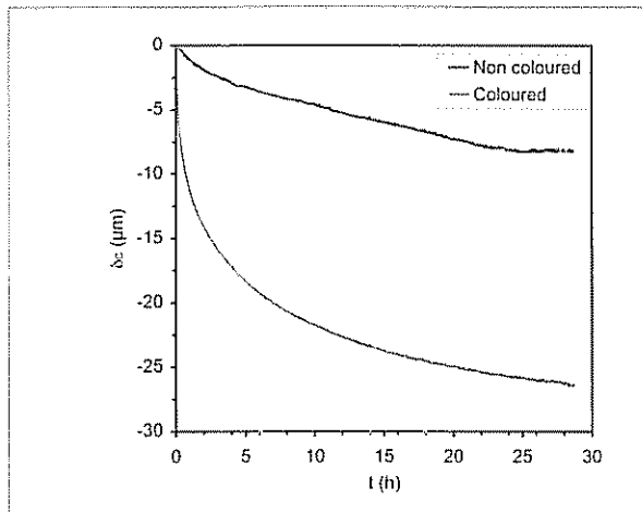
Fig. 18 Influence of dry colouring on creep
