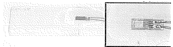
Fig. 8 Residual stress measurement test and detail of the gauge
