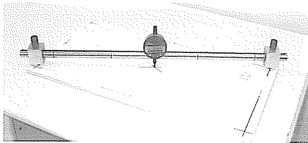
Fig. 1 Arrangement used to measure the deflection of industrial tiles
