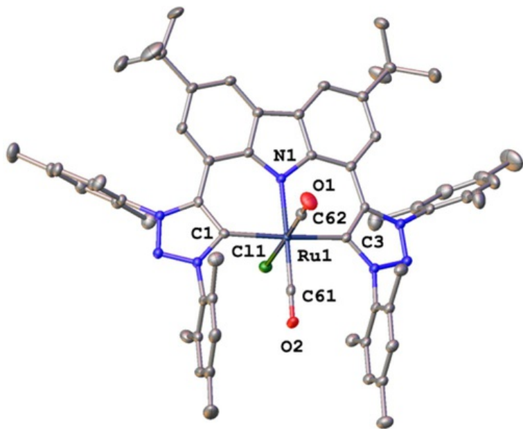
Fig. 2 Molecular structure of complex 1 with 50% probability ellipsoids. Hydrogens and one solvent molecule of \text{CH}_2\text{Cl}_2 have been omitted for clarity. Selected bond distances (Å) and bond angles ( ^\circ ): Ru(1)-C(1) = 2.132 (2); Ru(1)-C(3) = 2.119 (2); Ru(1)-N(1) = 2.1308 (17); Ru(1)-C(61) = 1.888(2); Ru(1)-C(62) = 1.853(2); Ru(1)-Cl(1) = 2.460(5); C(1)-Ru(1)-C(3) = 169.4(8) ; N(1)-Ru(1)-C(61) = 176.7(8) ; N(1)-Ru(1)-Cl(1) = 88.1(5)
