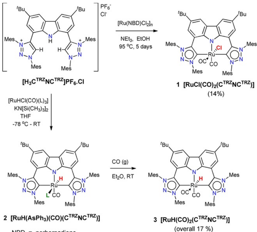
Scheme 1 Synthesis of complexes 1–3.
