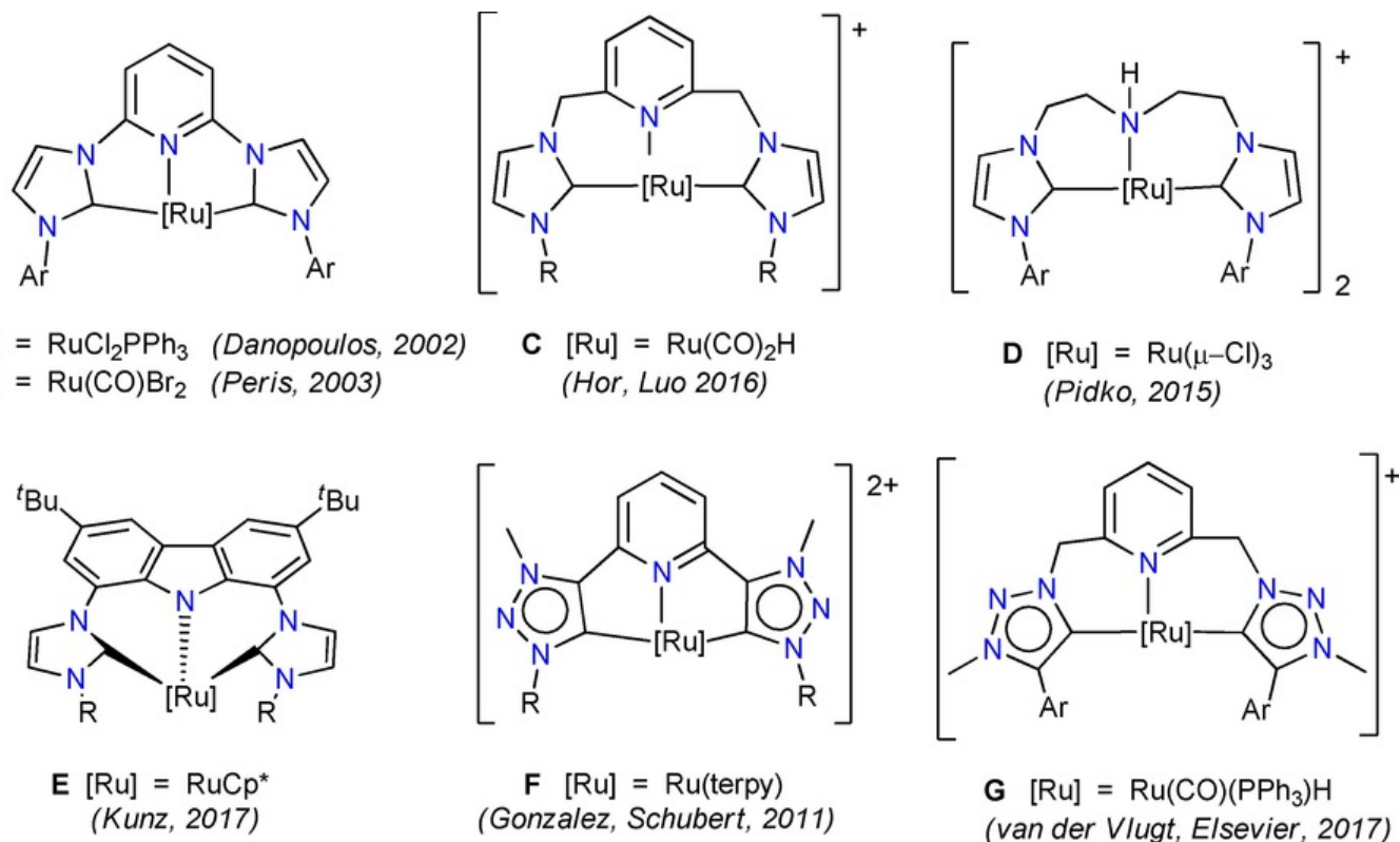
Fig. 1 Examples of previously reported carbene-based CNC-Ru(II) complexes.
