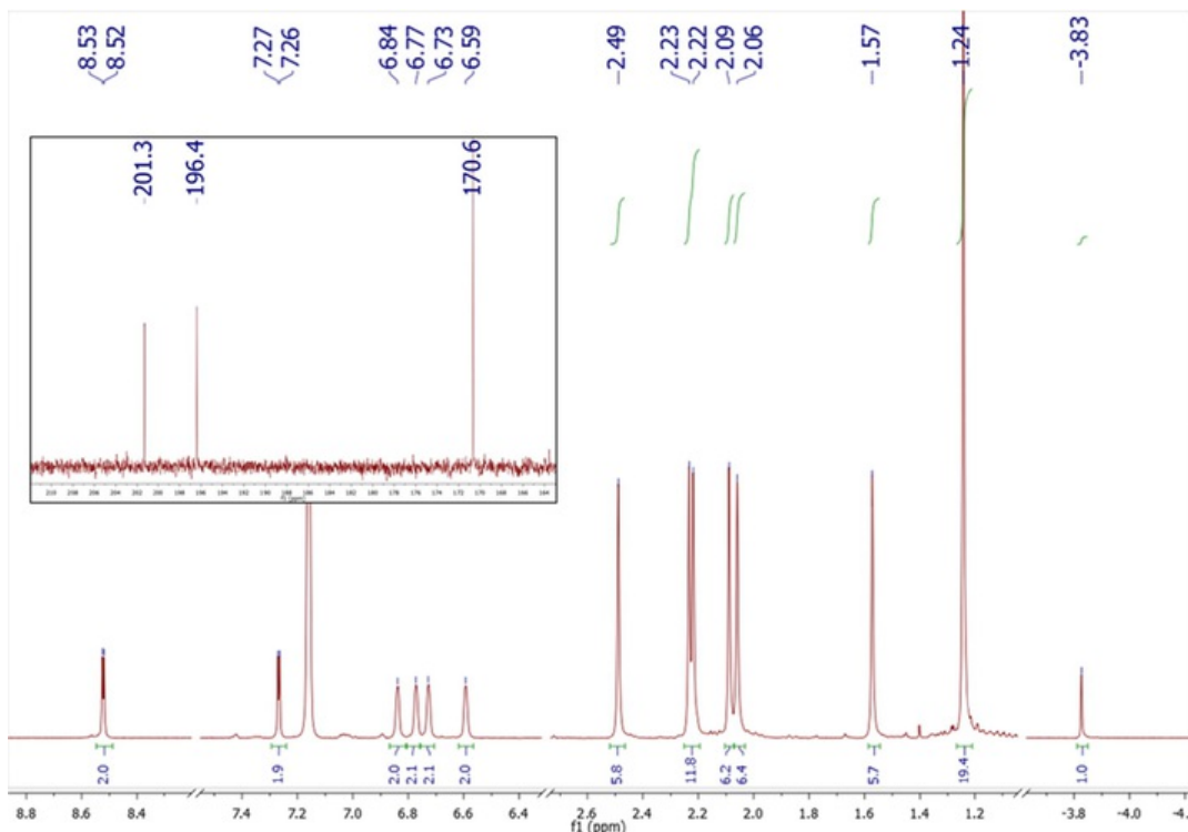
Fig. 3 ^1\text{H} and ^{13}\text{C} (inset) NMR spectrum of 3 .
