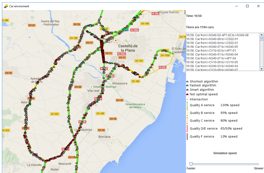
FIGURE 3.4: Graphical user interface
