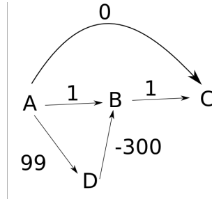
FIGURE 2.2: An unsolvable graph for Dijkstra
