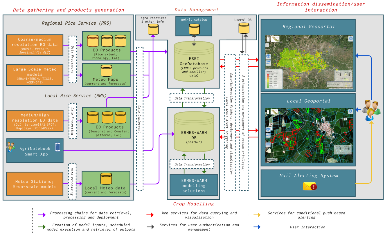
Fig. 2. Overall architecture of the ERMES system.
