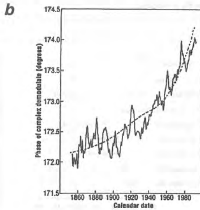
Fig. 12. Phase of the Jones-Wigley Northern Hemisphere land plus marine temperature series, Fig. 5, after a linear offset 50^{\circ}.256 . ( t - 1854 ) from precession has been added. It is thus an estimate of deviation of the phase from the trend in Fig. 5 that was observed in the early part of the record. The dashed line is a least-squares fit to the phase regressed on the logarithm of atmospheric \text{CO}_2 levels and a constant. For a significance test, see Fig. 13.
