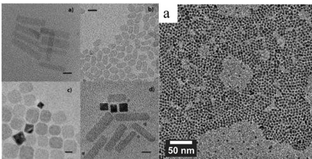
Figure 4. On the left, the transmission electron microscope images of CdSe colloidal nanoplalelets. Different lateral shapes (a-d) can be obtained using different precursors. Scale bars: b) 20nm, others, 10nm 2 . On the right, TEM images of bare CdSe quantum dots of average size 5 nm. 3
