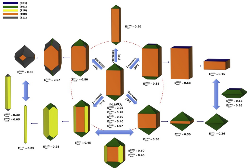
Fig. 2 Ideal morphology (in the center) and map of a few morphologies of t\text{-LaVO}_4 . Surface energy is in \text{J m}^{-2} .
