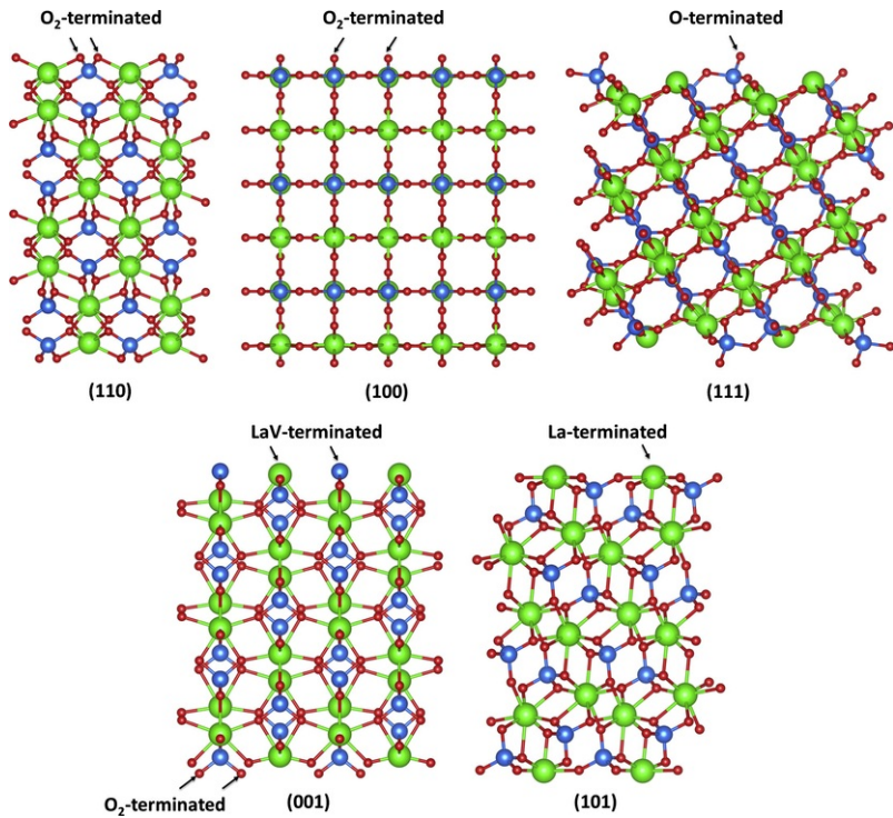
Fig. 1 Surface models of (1 1 0), (1 0 0), (1 1 1), (0 0 1) and (1 0 1) for t\text{-LaVO}_4 . The green, blue and red represent La, V and O atoms, respectively. (For interpretation of the references to color in this figure legend, the reader is referred to the web version of this article.)
