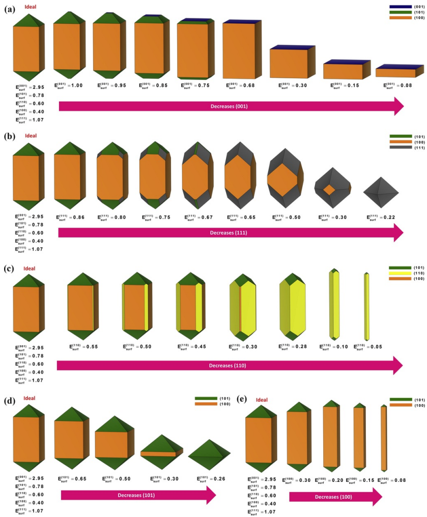
Fig. 3 Morphologies of t -LaVO 4 when the values of E_{surf} decrease for (a) the (0 0 1) surface; (b) the (1 1 1) surface; (c) the (1 1 0) surface; (d) the (1 0 1) surface and (e) the (1 0 0) surface. Surface energy is in J m -2 .
