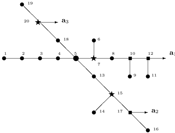
Fig. 2. Proximity and dual graphs of Example 1-1.B.
