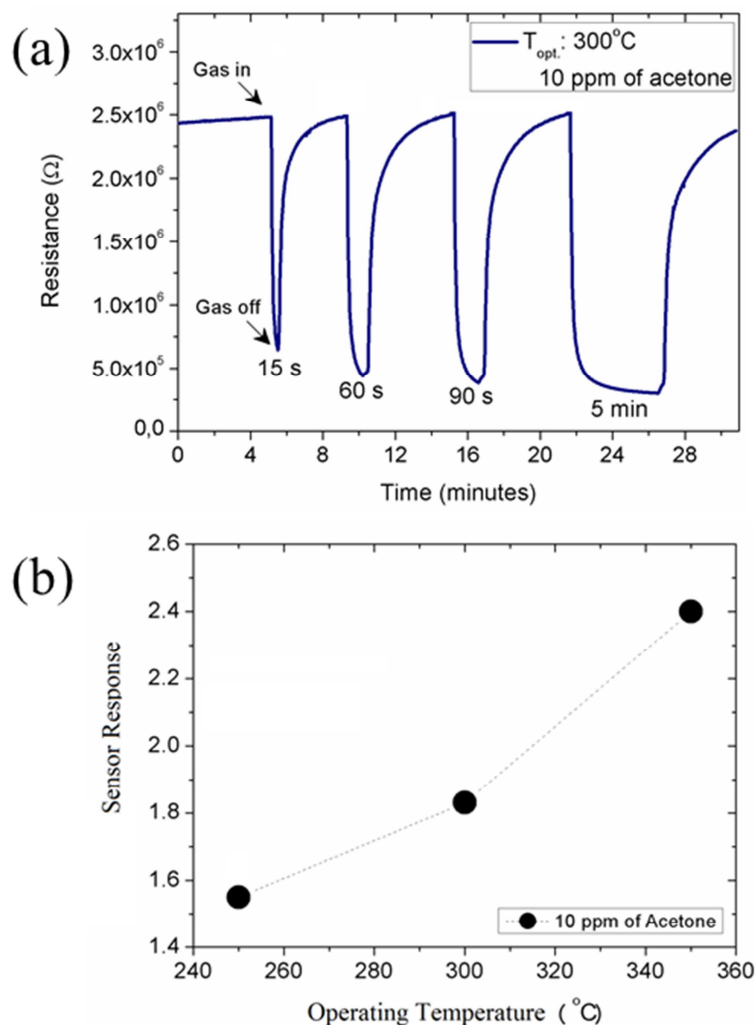
Fig. 2. (a) Electrical resistance of \alpha -Ag 2 WO 4 nanorods upon exposure to 10 ppm acetone for differing times at an operating temperature of 300 °C. (b) Sensor response vs. operating temperatures.
