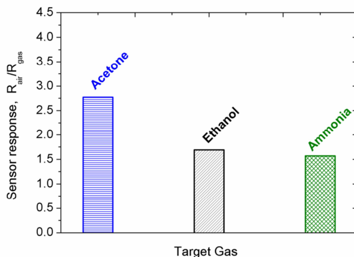
Fig. 4. Sensor response of the \alpha\text{-Ag}_2\text{WO}_4 nanorods towards acetone, ethanol, and ammonia.
