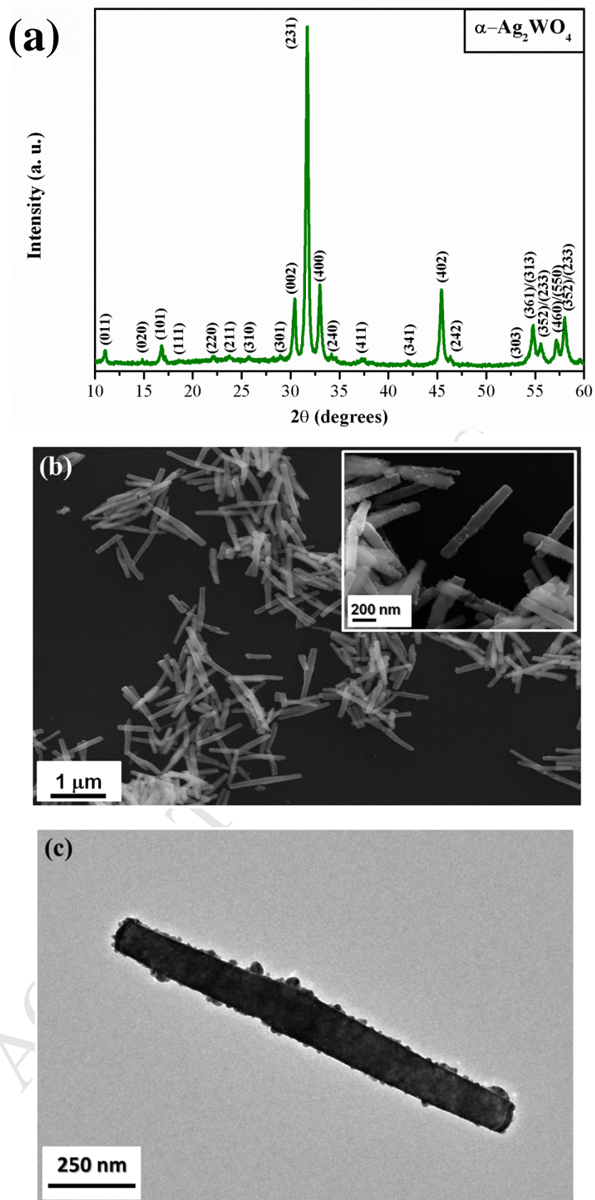
Fig. 1. The \alpha\text{-Ag}_2\text{WO}_4 sample prepared via MAH treatment method. (a) XRD pattern, (b) FESEM image, and (c) TEM image.
