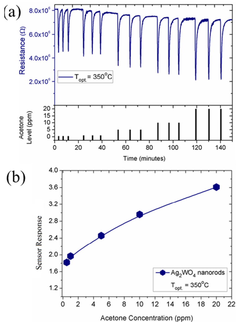
Fig. 3. Acetone gas-sensing response for the \alpha\text{-Ag}_2\text{WO}_4 nanorods. (a) Electrical resistance and (b) sensor response vs. acetone concentration at 350^\circ\text{C} .
