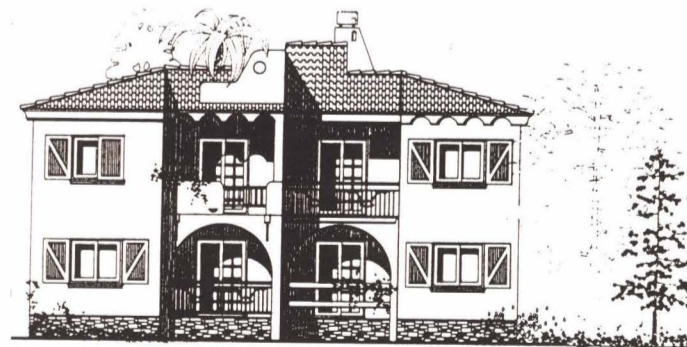
ALZADO PRINCIPAL
