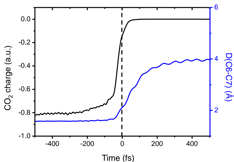
Figure 4. Averaged time evolution of the C6-C7 distance (blue) and the charge on the \text{CO}_2 leaving group (black) along reactive trajectories.
