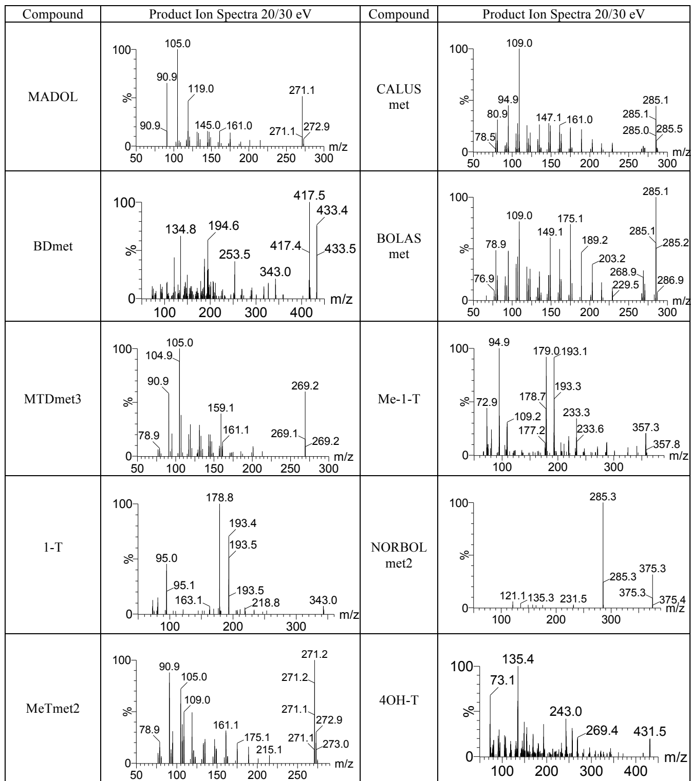
Figure S1. Product ion spectra of the selected compounds obtained at different collision energies
