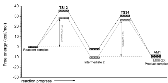
Figure 6. Free energy reaction pathway of the two steps mechanisms of hydrolysis of methyl acrylate catalyzed by PALB computed at AM1/MM (black line) and M06-2X/MM (grey line) level.
