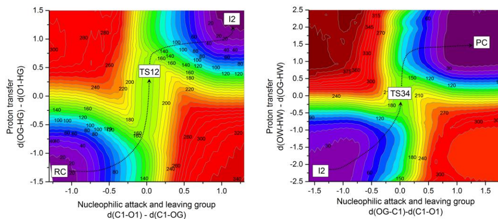
Figure S2. AM1/OPLS/TIP3P 2D-PMF surfaces for the reaction mechanism of hydrolysis of methyl acrylate catalyzed by PALB.
