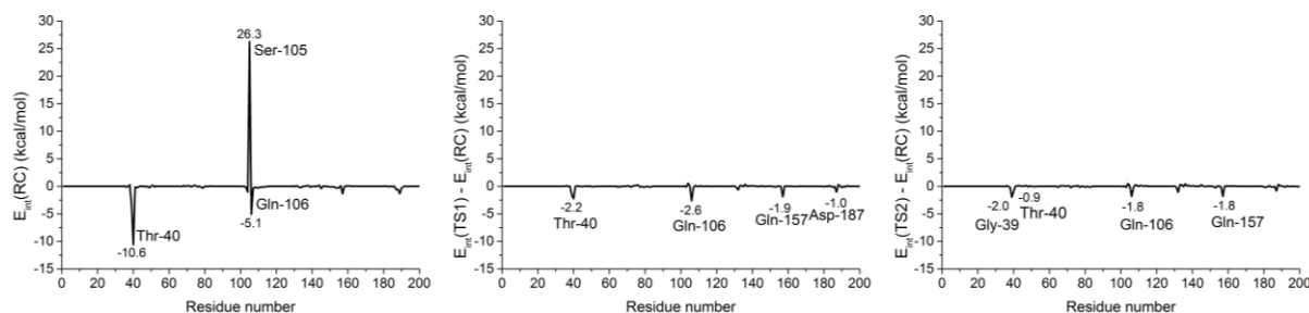
Figure 3. Averaged contributions of individual amino acids to substrate-protein interaction energies (in kcal mol -1 ), computed for RC, left panel, and difference between TS1 and RC (center panel) and TS2 and RC (right panel).
