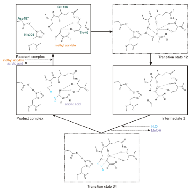
Figure 5. Two-step proposed reaction mechanism for hydrolysis of methyl acrylate catalyzed by PALB.
