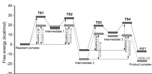
Figure 4. Free energy profile for the multi-step reaction mechanism of hydrolysis of methyl acrylate catalyzed by PALB obtained at M06-2X/OPLS/TIP3P (in grey) and AM1/OPLS/TIP3P (in black).
