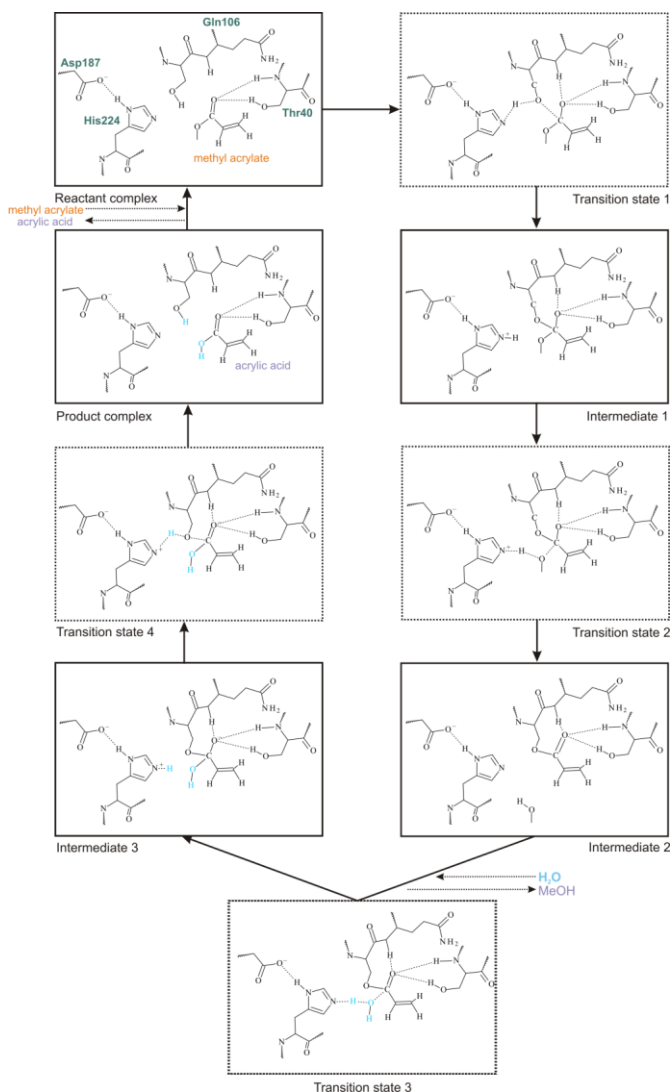
Figure 2. Multi-step proposed reaction mechanism for hydrolysis of methyl acrylate to acrylic acid and methanol, catalyzed by PALB.
