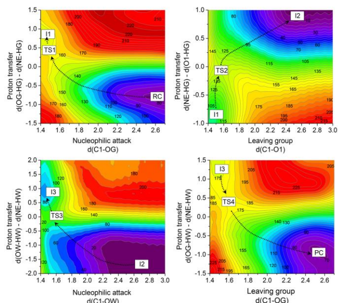
Figure 1. M06-2X//OPLS/TIP3P 2D-PMF surfaces for the reaction mechanism of hydrolysis of methyl acrylate catalyzed by PALB.
