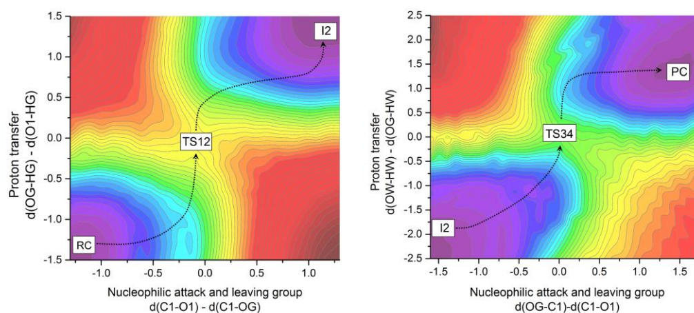
Figure S1. AM1/OPLS/TIP3P PESs for the reaction mechanism of hydrolysis of methyl acrylate catalyzed by PALB.
