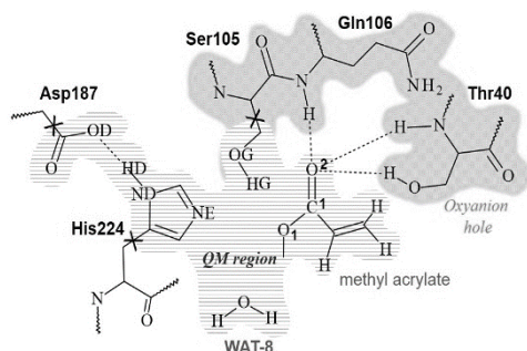
Scheme 1. Representation of the active site of PALB together with bound methyl acrylate substrate. Light grey shaded region contains atoms treated quantum mechanically. Oxyanion hole are highlighted in dark grey. Quantum link atoms are represented as crosses.
