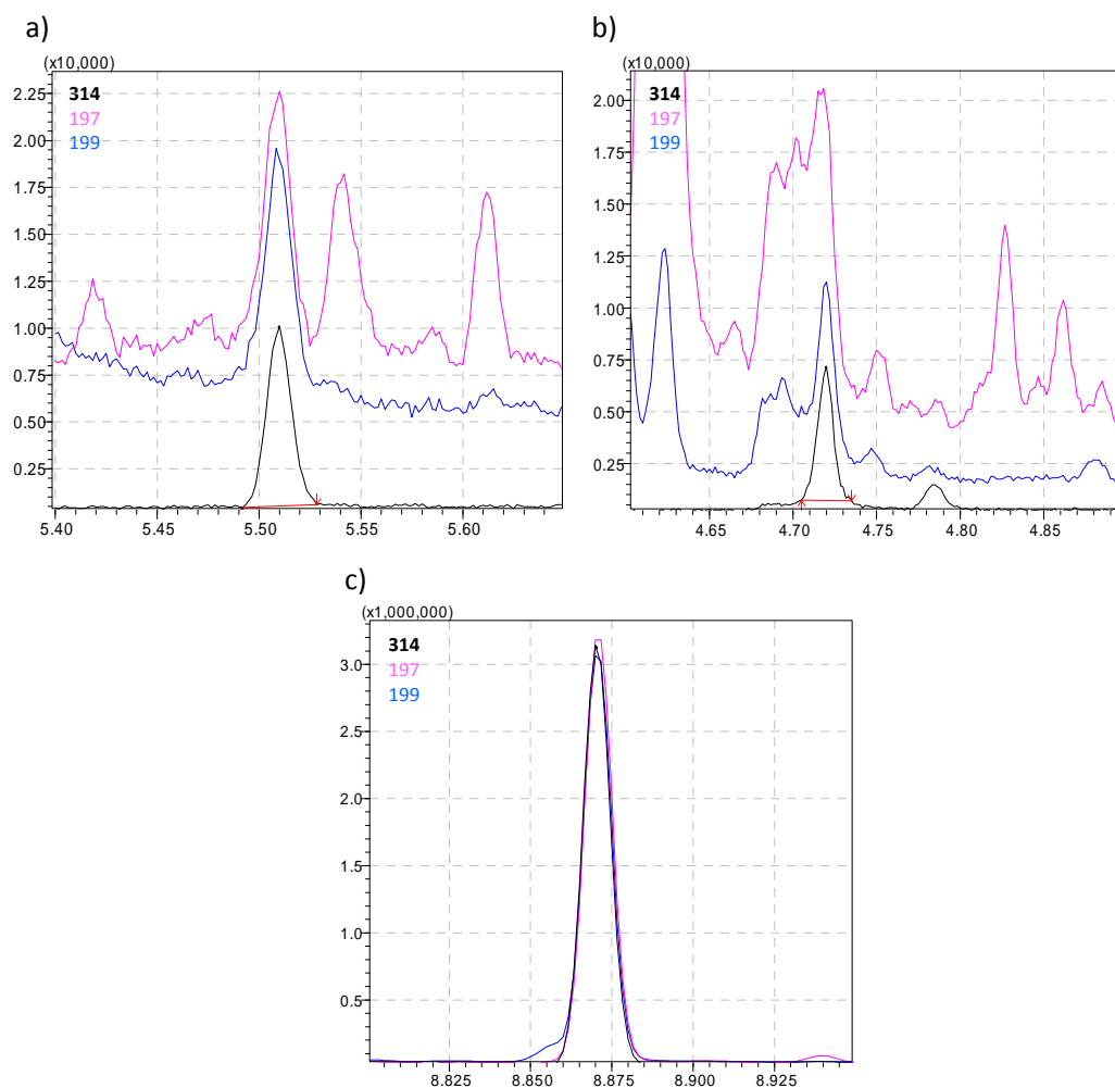
Fig 5. Comparison of chromatographic responses for chlorpyrifos in apple juice extract spiked at 0.01 mg/L after applying a QuEChERS, b SPE, and c SPME. Target ion ( bold ) and two reference ions are shown.
