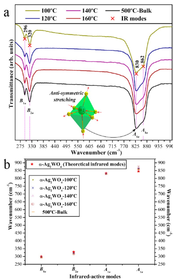
Figure 3. (a) FTIR spectra of \alpha - \text{Ag}_2\text{WO}_4 prepared at different temperatures (100, 120, 140, and 160 °C) for 1 h by the MAH method. The vertical lines indicate the relative positions of the infrared-active modes. (b) Comparison between the theoretical and experimental infrared-active modes from 250 to 900 \text{cm}^{-1} .
