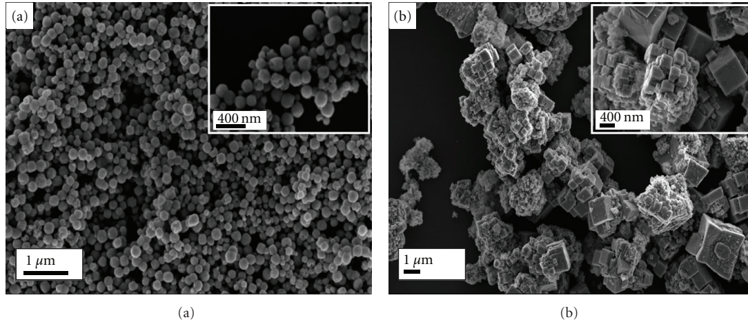
FIGURE 2: FE-SEM images of SrTiO 3 powders obtained with different precursors: (a) SAM1 and (b) SAM2 samples.
