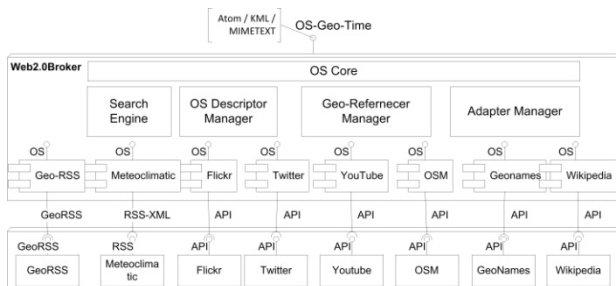
Figure 2: W2.0B components diagram.
