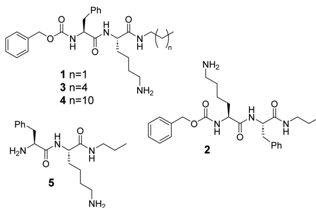
Fig. 1 Structure of L-lysine-based dipeptides 1–5.
