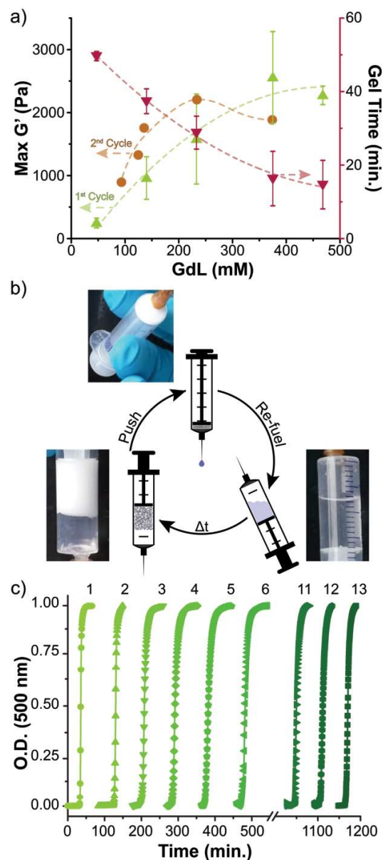
Figure 3. Rheology and syneresis experiments. (a) Rheology showing a trend of decreasing gelation time ( \blacktriangledown ) and increasing stiffness ( G' - \blacktriangle ) with increasing [GdL] for solution to gel transition in the transient cycles. [HMTA] = 190 mM, [DT] = 191 mM, [SachCHO] = 54 mM. Resetting of hydrogels after the first cycle ([HMTA] = 95 mM, [DT] = 96 mM, [GdL] = 93.6 mM, [SachCHO] = 54 mM) by second round of fuels addition ([HMTA] = 190 mM, [DT] = 96 mM) with similar [GdL]-dependent stiffness trend ( \bullet ) (dashed lines are to guide the eye). Error bars show standard deviations over three independent experiments, whereas circles depict single measurements. (b) In clockwise direction, chemically fueled gel made in a syringe (bottom left), fiber network remains in the syringe after solvent expulsion by pushing the plunger (top), dissolution of fibers after refueling (bottom right), and re-formation of gel after a defined
