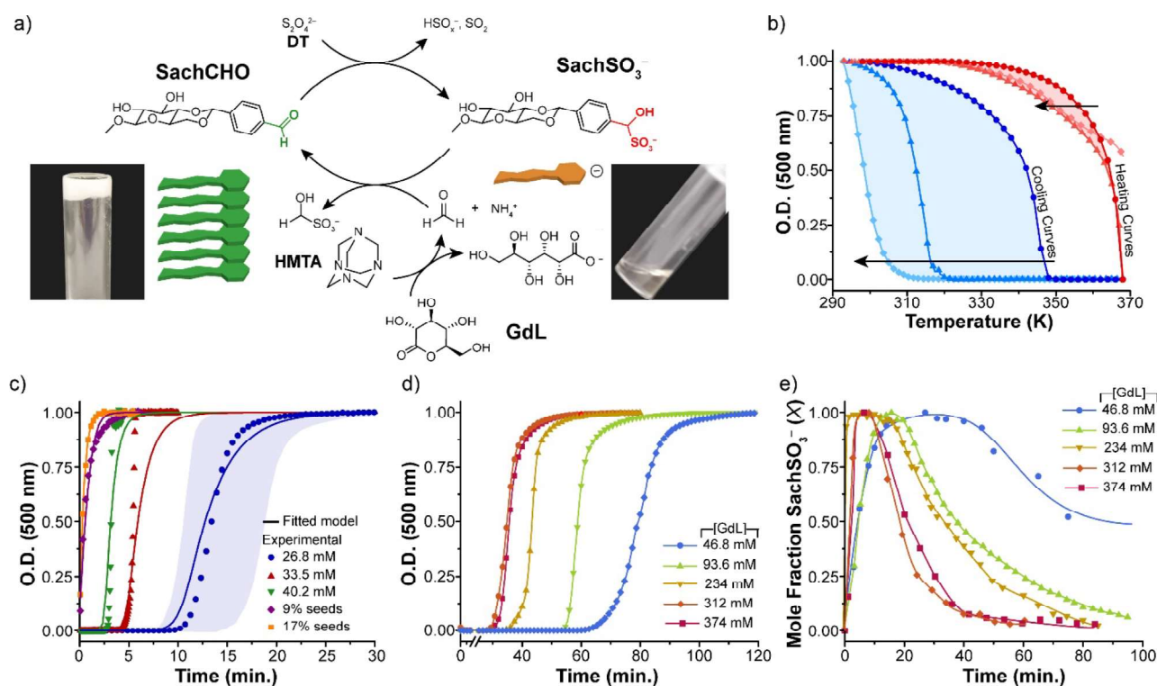
Figure 1. (a) Scheme of the chemically fueled reaction cycle for transient disassembly by dithionite DT of SachCHO hydrogelator followed by in situ catalytic formation of formaldehyde by glucono- \delta -lactone GdL and hexamethylenetetramine HMTA, leading to re-gelation. (b) Heat-cool cycles at different rates for thermally annealed gel using UV-Vis turbidity measurements, where the optical density (O.D.) at 500 nm is measured. 70 degree, 50 degree and 20 degree hysteresis for heat/cool rate 10 K/min ( \blacklozenge ), 1 K/min ( \blacktriangle ), and 5 min hold at each temperature ( \bullet ), respectively. Arrows represent increasing heating/cooling rate. (c) Global fitting of (un)seeded gelation (SachSO 3 - to SachCHO) using excess HCHO followed using O.D. at 500 nm (see main text). Legend shows initial [SachSO 3 - ]. The faded blue region delineates the upper / lower boundaries of triplicate experiments. (d) O.D. at 500 nm for SachSO 3 - solution to SachCHO gel, catalyzed at different [GdL]. Lines to guide the eye. (e) Evolution of SachSO 3 - in the transient cycles as seen by NMR. Lines to guide eye. Initial thermal gel with [SachCHO] = 54 mM, and [HMTA] = 190 mM, [DT] = 191 mM in chemically fueled transient cycles.
