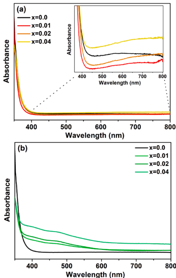
Fig. 4. Optical absorbance spectra of (a) \text{Zn}_{1-x}\text{Ni}_x\text{O} and (b) \text{Zn}_{1-x}\text{Fe}_x\text{O} ( x=0.01 ; 0.02 and 0.04 mol) samples obtained by the MAH method, x= mol of \text{Ni}^{2+} or \text{Fe}^{3+} .
