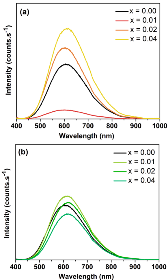
Fig. 5. PL spectra of (a) \text{Zn}_{1-x}\text{Ni}_x\text{O} and (b) \text{Zn}_{1-x}\text{Fe}_x\text{O} ( x=0.01 ; 0.02 and 0.04 mol) samples at room temperature ( \lambda_{\text{exc}}=355\text{ nm} ) prepared by the MAH method; x= mol of \text{Ni}^{2+} or \text{Fe}^{3+} .
