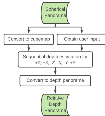
Fig. 7 Overview of depth estimation process
