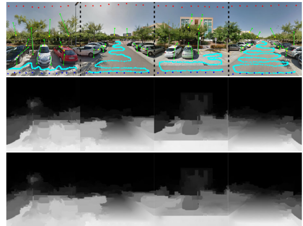
Fig. 6 Depth maps for the left, front, right and back faces of a cube map: Provided input (top), using DfSI separately (center) and using our method (bottom). There are depth discontinuities in boundaries when DfSI is applied separately
