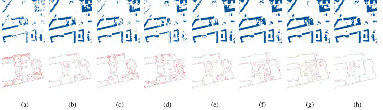
Fig. 4. ISPRS Potsdam dataset: the top row displays the predicted building masks and the bottom row displays the generated building boundaries of one area, where red, green and blue colors denote the FP, TP and FN, respectively: (a) CE; (b) Dice; (c) NR-Dice; (d) CE_Dice; (e) ELL; (f) WDice; (g) BD_Dice; (h) BD_LACE_WDice. (Better to view zoom-in.)
