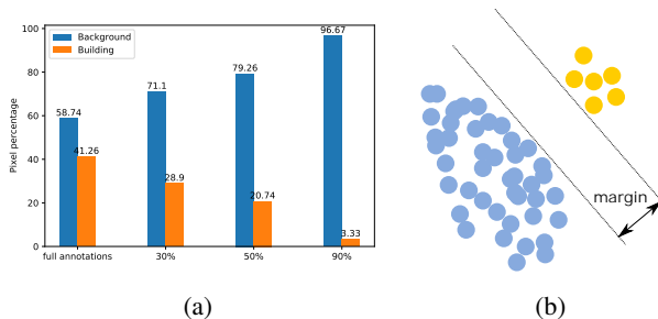
Fig. 2. (a) The background and building pixel percentages of the Massachusetts Buildings dataset with the full, 70%, 50% and 10% building annotations. (b) LACE tries to set a pairwise label margin between the predicted scores between majority and minority classes.
