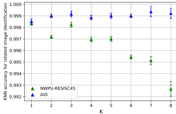
Fig. 6. KNN-based classification of rotated image identification when K = 1, 2, 3, 4, 5, 6, 7, 8 on the two rotation-augmented datasets with the angles of [0^\circ, 45^\circ, 90^\circ, 135^\circ, 180^\circ, 225^\circ, 270^\circ, 315^\circ] .
