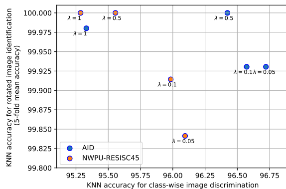
Fig. 7. Sensitivity analysis of parameter \lambda based on KNN classification of both rotated image identification and class-wise image discrimination, when \lambda = 0.05, 0.1, 0.5, 1 .
