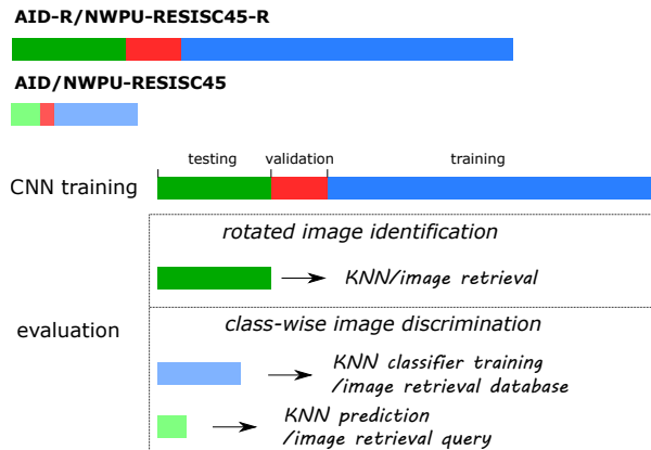
Fig. 4. A simplified graphical illustration describing the configuration of datasets in our experiments
