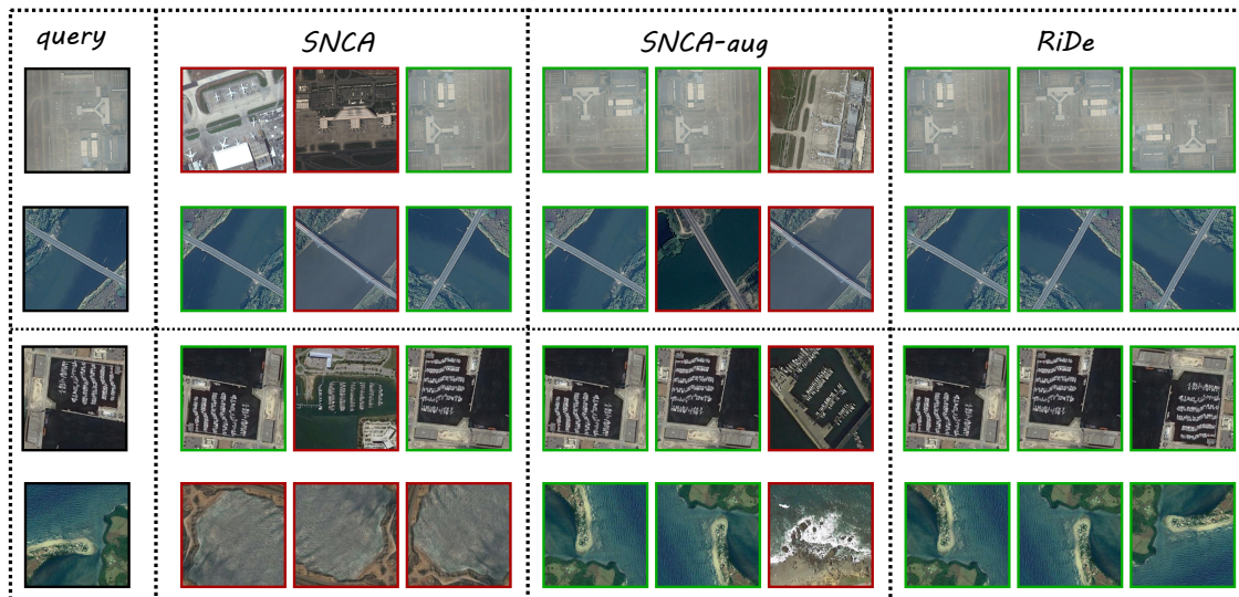
Fig. 5. For different query images, we display the three nearest neighbors retrieved from the test sets of AID-R (first two rows) and NWPU-RESISC45-R (last two rows), based on the deep embeddings extracted from the trained ResNet50 via SNCA, SNCA-aug and RiDe. The images not rotated from the same source image are marked in red color, while the images rotated from the same source image are marked in green color.
