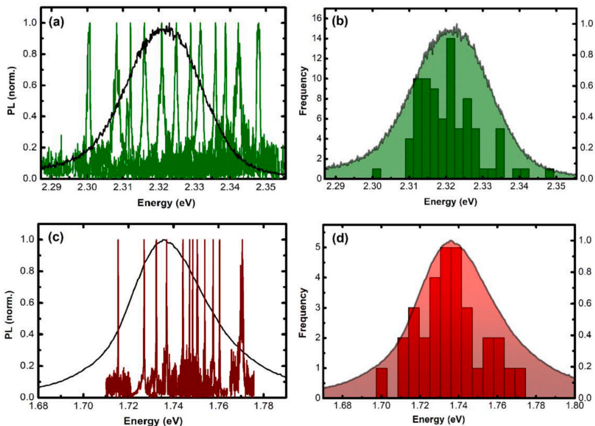
Fig. 3. (a–c) Representative micro-PL spectra at 4 K of CsPbBr 3 (green curves) and CsPbI 3 (brown curves) PNCs as compared to the PL spectra (black curves) of the corresponding high-density samples. (b–d) Statistics obtained for the micro-PL peak energies in around 80 CsPbBr 3 (green histogram) and more than 30 CsPbI 3 (red histogram) single PNCs. Green and red shadowed curves in (b–d) are the same reference PL spectra as in (a–c).
