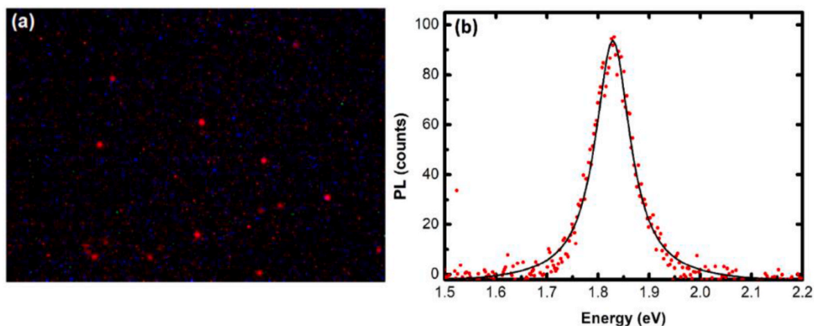
Fig. 2. (a) Typical image captured with the microscope camera, (b) A representative micro-PL spectrum of one of the CsPbI 3 PNCs (red dotted curves) in a fresh sample at RT, along with the Lorentzian fit (continuous black curves).
