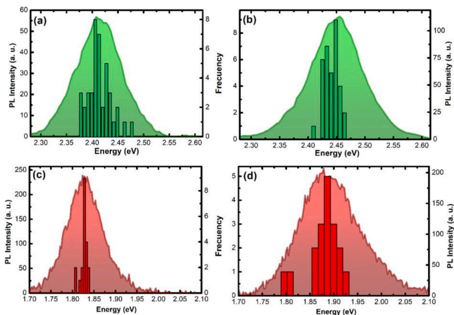
Fig. 4. (a–c) Histograms of peak energies extracted from micro-PL spectra measured at RT in 41 (green color) and 20 (red color) of CsPbBr 3 (a) and CsPbI 3 (c) PNCs (first synthesis) in fresh samples, respectively. (b–d) idem for the case of 34 and 18 PNCs of the same samples measured next day. In all cases, representative homogeneous micro-PL spectra (similar to those in Figs. 1 and 2) are plotted as green- and red-shaded curves for CsPbBr 3 (a–b) and CsPbI 3 (c–d).
