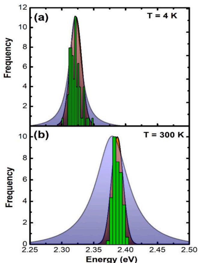
Fig. 7. Comparison of normalized PL spectra (shaded in blue) 4 K (a) and RT (b) for the high-density layer of CsPbBr 3 PNCs (second synthesis) as compared to the histograms (green bars) of micro-PL peak energies extracted from measurements in the sample just after preparation at 4 K (a) and RT (b) using the same CsPbBr 3 PNCs (second synthesis). Red shaded curves stand for the calculated (Equation S6) emission shape expected from the size histogram in these PNCs (Figure S1d).
