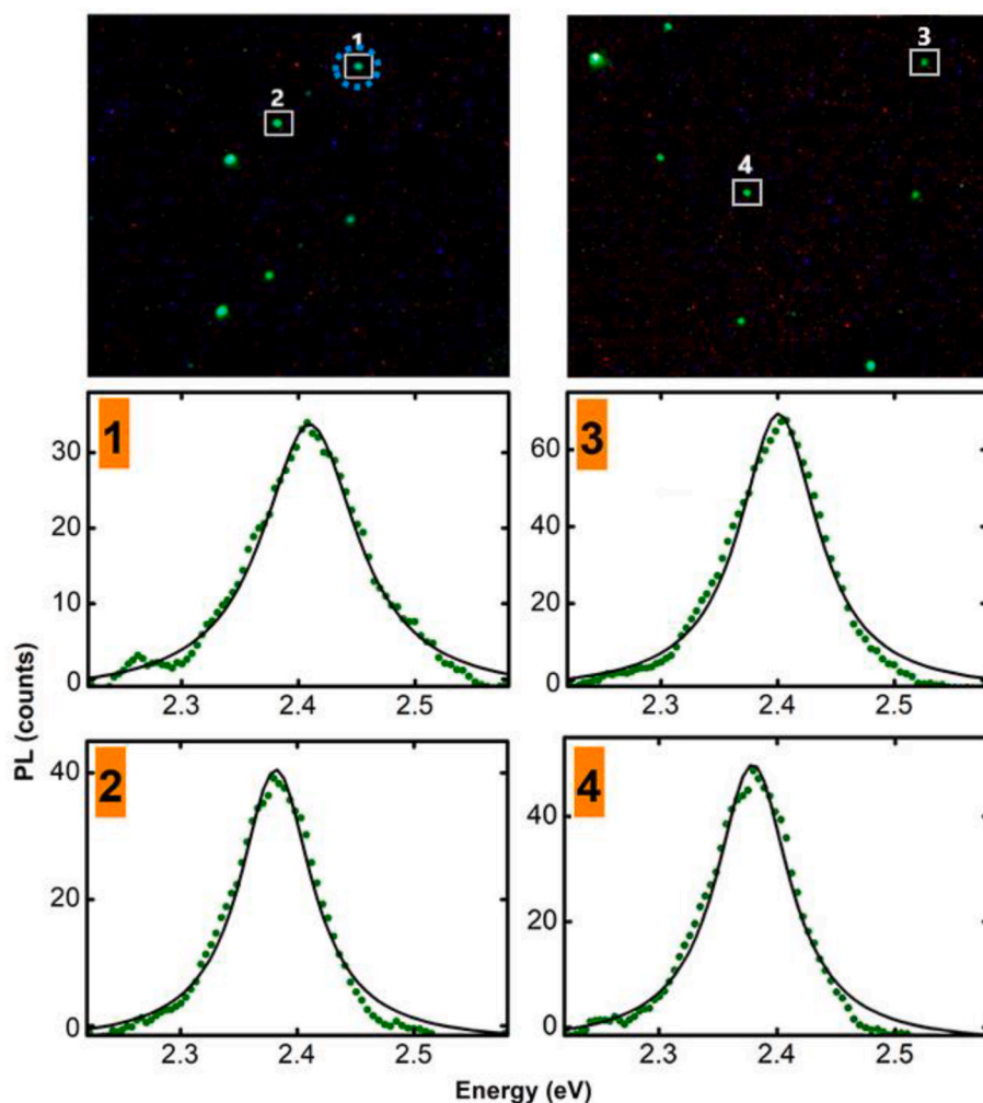
Fig. 1. (top panels) Micro-PL images at room temperature captured with the C-MOS camera (2s exposure) from two different regions of the sample containing \text{CsPbBr}_3 PNCs emitting at green wavelengths (green circles that have been boxed and marked with numbers 1 to 4). These circles of green light have a repetition image beneath them, due to the second surface of the quartz plate (1 mm thick) that is being used as a signal beam splitter. The different single-color points observed in the images correspond to individual pixels of the camera due to background noise. (bottom panels) Experimental micro-PL spectra (green dotted lines) corresponding to the \text{CsPbBr}_3 PNCs selected in top panels. Continuous lines stand for a Lorentzian shape fitting, as explained in the text.
