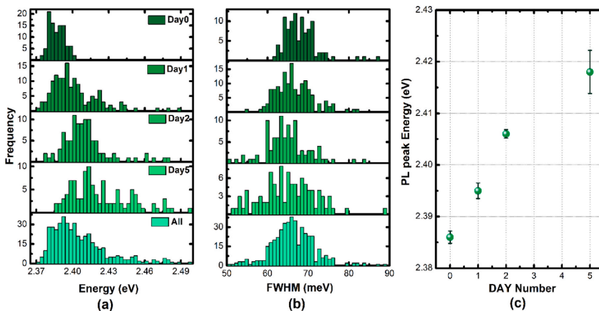
Fig. 5. Histograms regarding micro-PL statistics for peak energies (a) and FWHM (b), magnitudes that were extracted from micro-PL spectra measured at RT in around 100 CsPbBr 3 PNCs (from the second synthesis) of the same sample, but measured immediately after preparation (Day0), one (Day 1), two (Day 2) and five days after preparation (Day 5), respectively. (c) Dependence of the average micro-PL peak energy with aging time, as extracted from the frequency histograms in (a).
