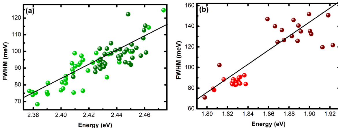
Fig. 6. Linear correlation between FWHM and peak energy extracted from its micro-PL spectrum in the 75 and 38 PNCs of CsPbBr 3 (a) and CsPbI 3 (b), respectively, studied in the present work. The experimental data points in light green and red (dark green and brown) correspond to the samples of CsPbBr 3 and CsPbI 3 measured immediately (next day) after preparation, respectively, together with the best fits to a straight line (black continuous line).
