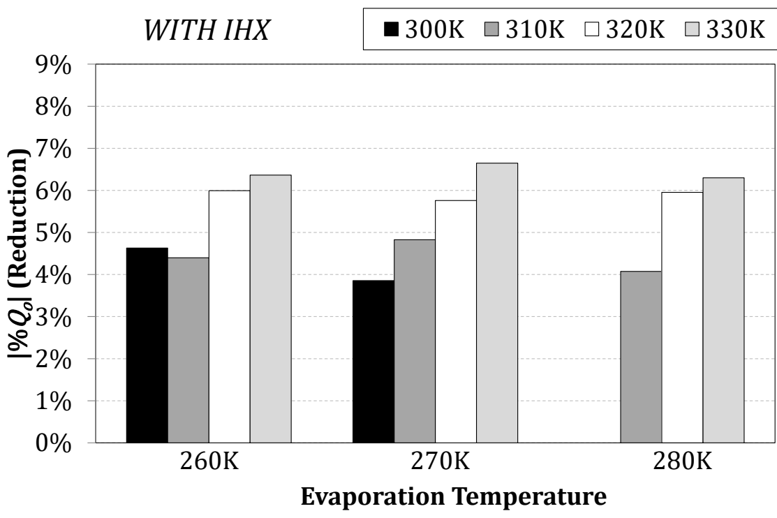
Figure 2. Cooling capacity relative reduction taking R134a as baseline a) with IHX and b) without IHX.
