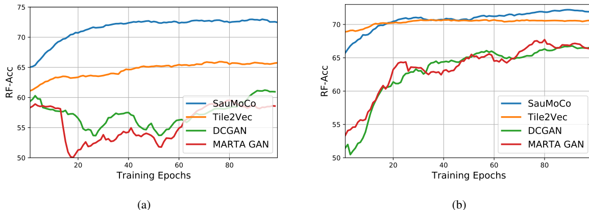
Fig. 4. RF classification performances based on the deep embeddings extracted from the NAIP (a) and EuroSAT (b) datasets via the proposed method (SauMoCo), Tile2Vec, and DCGAN (during the training phase).
