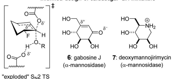
Fig. 1 Panel (A): currently accepted mechanism for the formation of the covalently bound glycosyl–enzyme intermediate in retaining glycoside hydrolases. Panel (B): structures of the iminosugar and carbasugar competitive inhibitors of glycoside hydrolases, deoxyfucojirimycin (1), 4- epi -isofagomine (2), and validamine (3). Panel (C): GH covalent inhibitor 4, its hydrolysis product 5, and the structure of the enzyme-intermediate with the T. maritima \alpha -galactosidase. Panel (D): depiction of the TS for covalent labeling of TmGalA , and the structures of GH inhibitors gabosine J (6) and deoxymannojirimycin (7).
