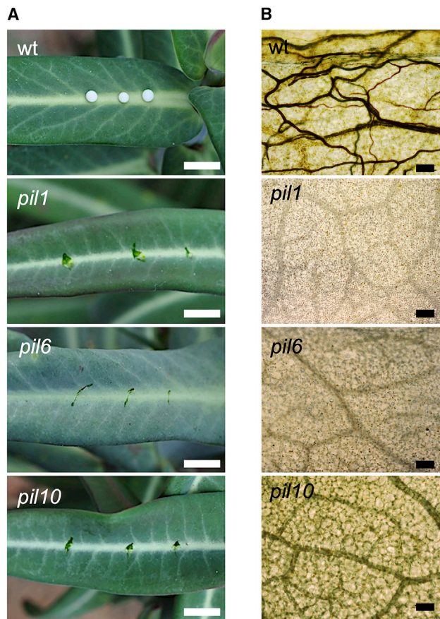
Figure 1. E. lathyris Mutants Used in This Study.
