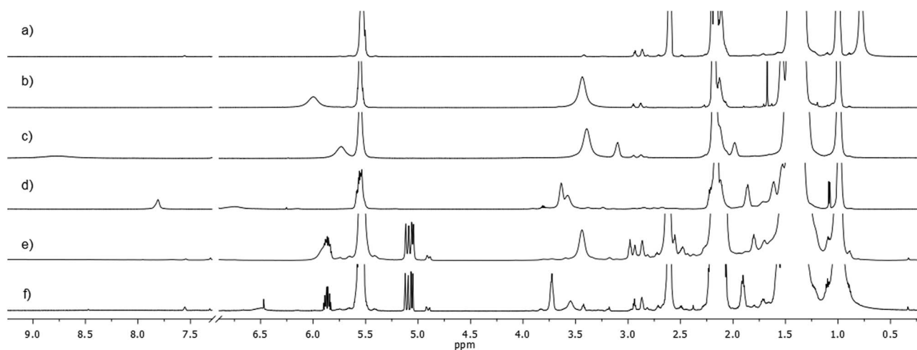
Fig. 3 (a–f) 1 H NMR spectrum (600 MHz, toluene- d 8 , 25 °C) of: (a) pure OLAM; (b) CS 2 /OLAm 1 : 2 (130 °C, 1 h); (c) WCl 6 /CS 2 /OLAm 0.25 : 4 : 8 (130 °C, 1 h); (d) WCl 6 /ODE/OLAm/CS 2 under 3–5 nm WS 2 NFL synthetic conditions (0.25 : 3 : 3 : 1; 130 °C, 1 h); (e) WCl 6 /ODE/OLAm/CS 2 under 3–5 nm WS 2 NFL synthetic conditions (0.25 : 3 : 3 : 1; 250 °C, 2 h).
