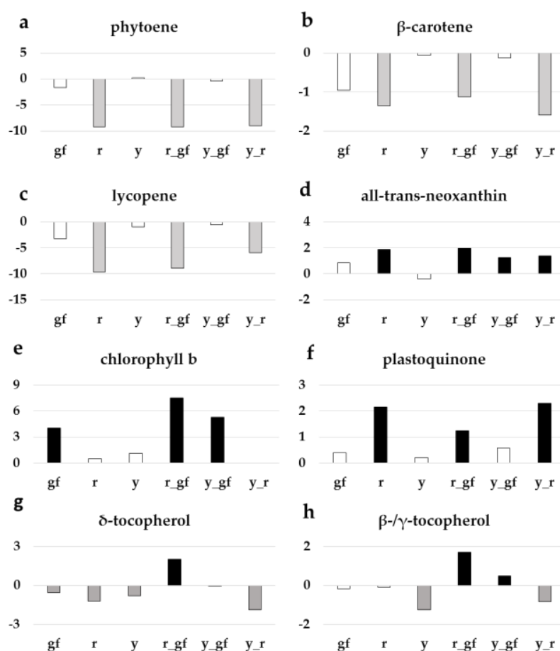
Figure 5. Relative log 2 variation in (a) phytoene, (b) β-carotene, (c) lycopene, (d) all-trans-neoxanthin, (e) chlorophyll b, (f) plastoquinone, (g) δ-tocopherol, (h) β-/γ-tocopherol, of six fruit mutant lines in San Marzano (SM) background compared with the recurrent parent. Line symbols are reported in Table 1. Bars colored in grey and black indicate means significantly lower and higher than SM for p \leq 0.05 after Student's t -test, respectively.
