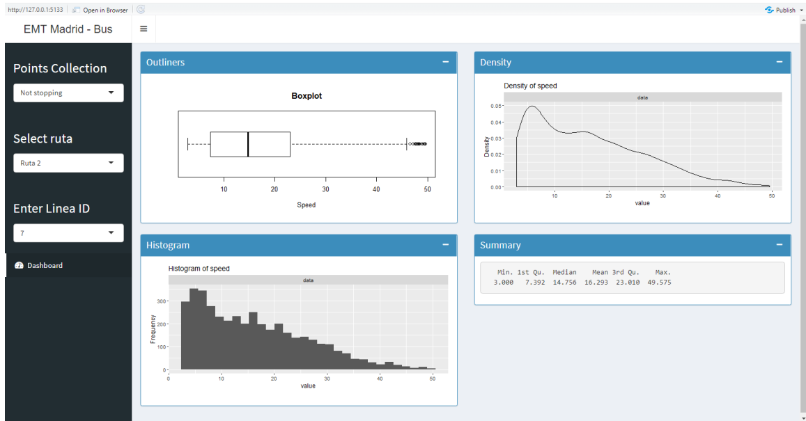
Figure 4.10: Shiny application that compare the speed from the points according to [Uno et al. 2009] approach.
