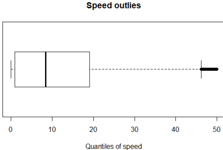
Figure 4.5: Speed outliers.
