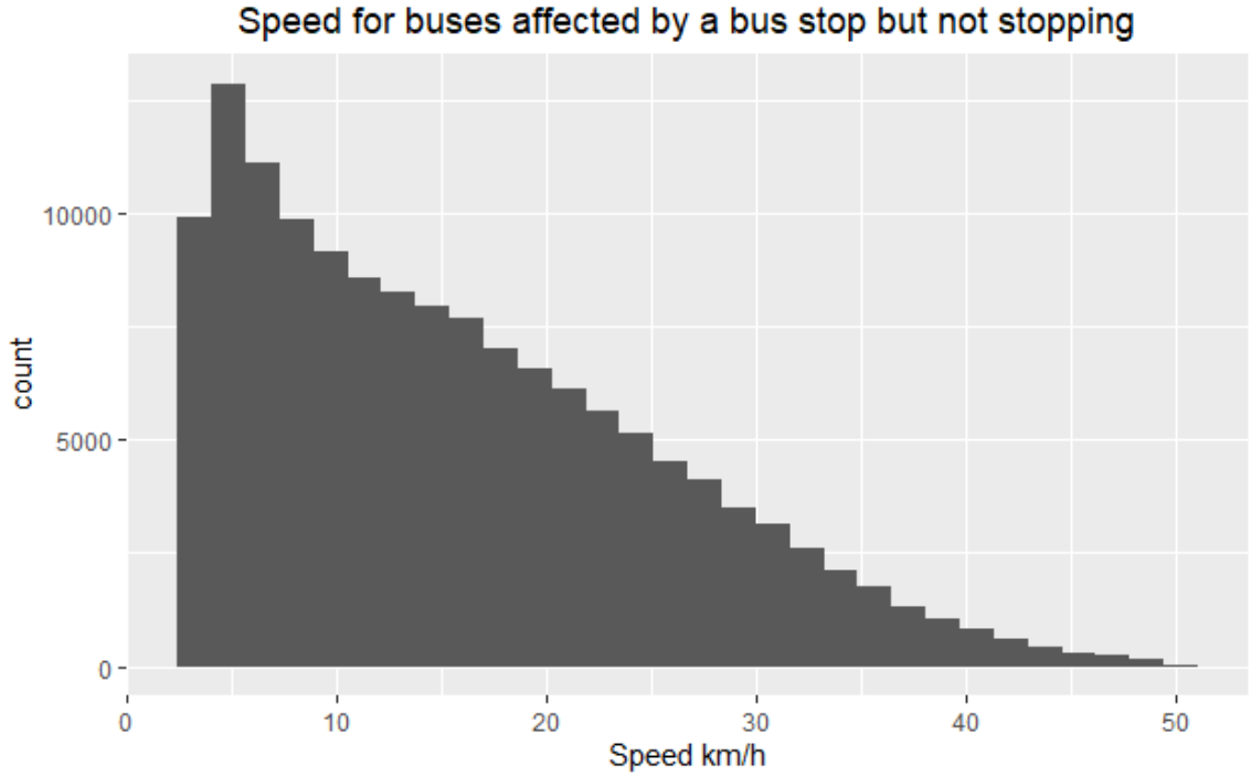
Figure 4.8: Speed for buses affected by a bus stop but not stopping on it.
