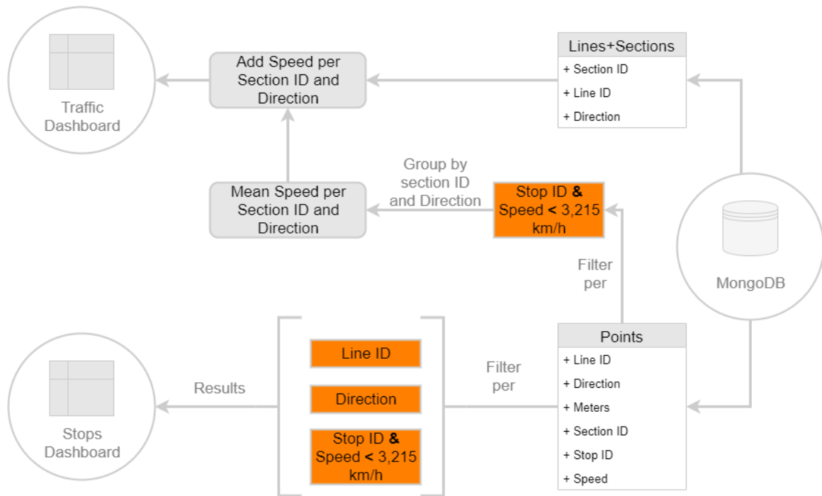
Figure 4.9: Shiny methodology.
