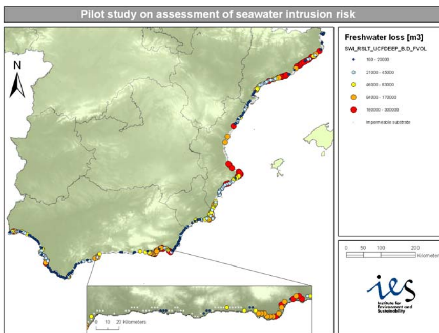
Figure 15: Absolute freshwater loss during transition from unstressed to stressed state. Results are displayed for simulations falling into the transient intrusion risk class only.
