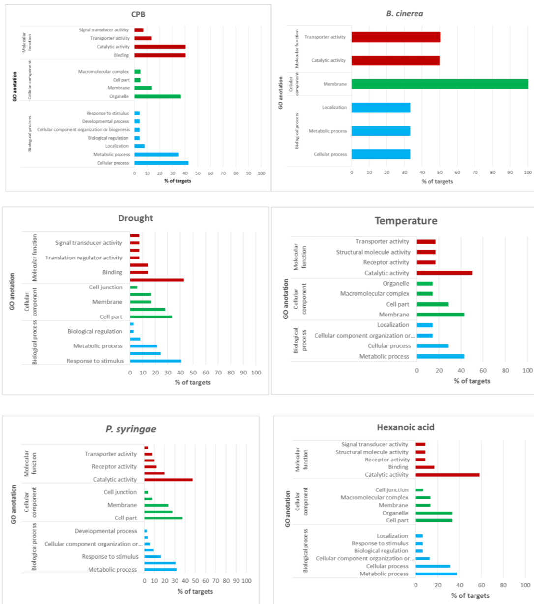
Figure 7. GO analysis of target transcripts regulated by stress-responsive miRNAs.
