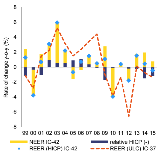
Graph 2.1.1: Evolution of price competitiveness in Spain
