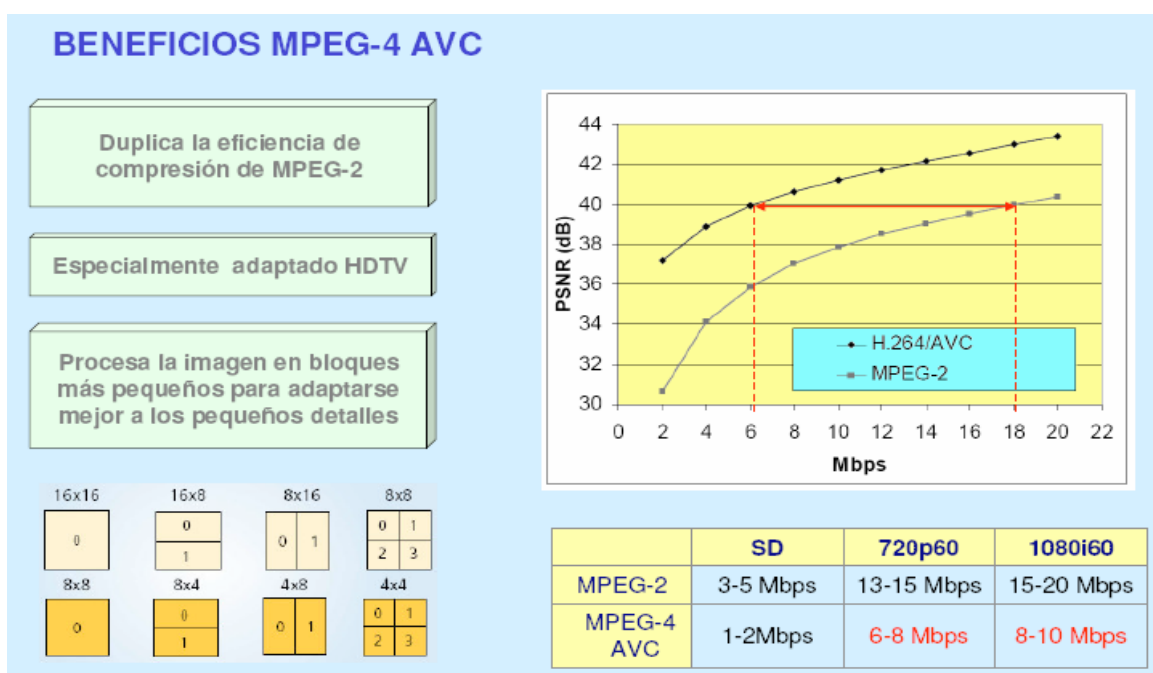
Figure 67. AVC Compression Algorithm ( www.vcodex.com )
