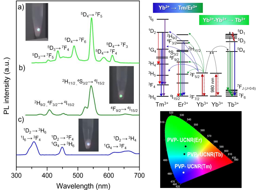
Figure 4. Left: Images of the emission in powdered samples and relative UC emission spectra for water suspensions of a) PVP-UCNR(Tb), b) PVP-UCNR(Er) and c) PVP-UCNR(Tm) under 980-nm diode laser excitation. Right: Proposed energy transfer mechanisms in the Yb:NaYF 4 nanorods codoped with Tm 3+ , Er 3+ and Tb 3+ . The full arrows represent photon excitation and emission processes; while dotted and dashed arrows represent energy transfer and multiphonon relaxation processes, respectively. Corresponding CIE chromaticity coordinates of the UCNRs.
