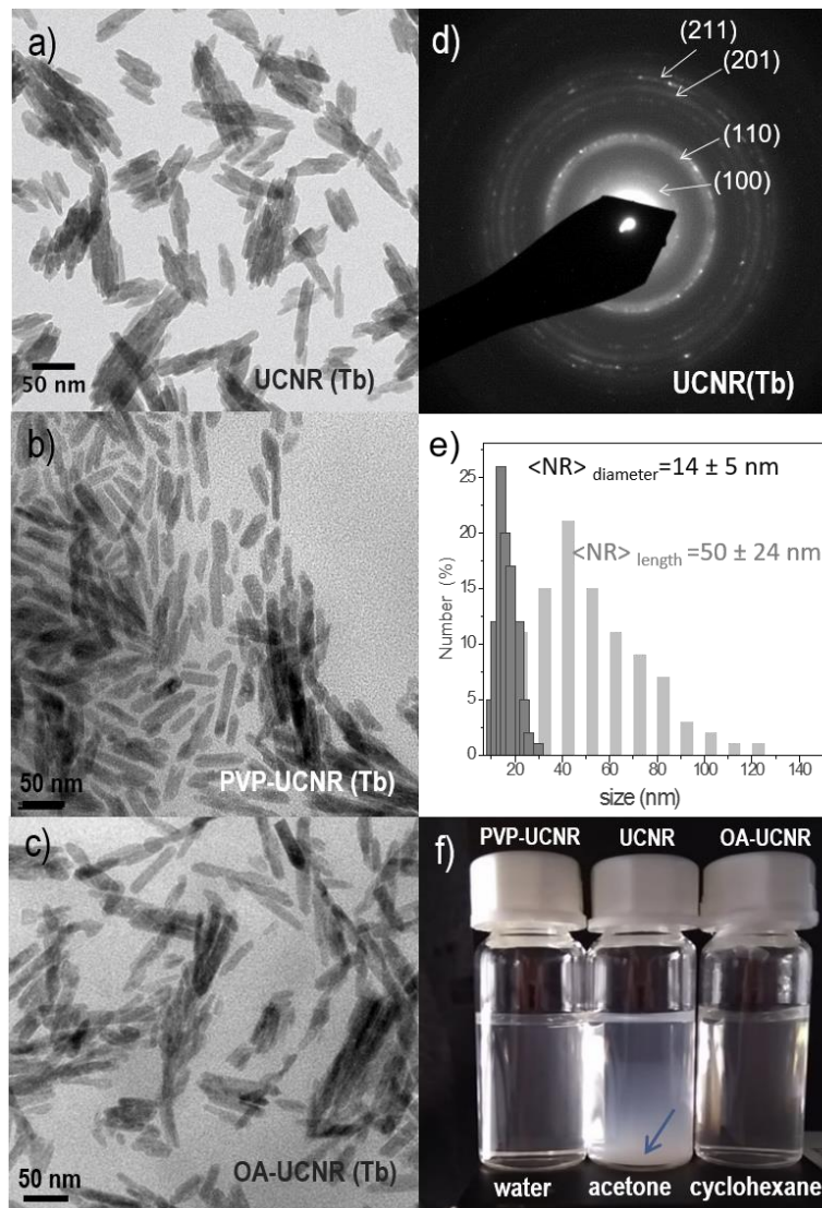
Figure 2. a,b,c) TEM images of the bare, PVP-coated and OA-coated UCNRs, respectively; d) SAED image from bare Tb-NRs; e) transversal and longitudinal size distribution of Tb-NRs; f) dispersion of the Tb-NRs in different solvents.
