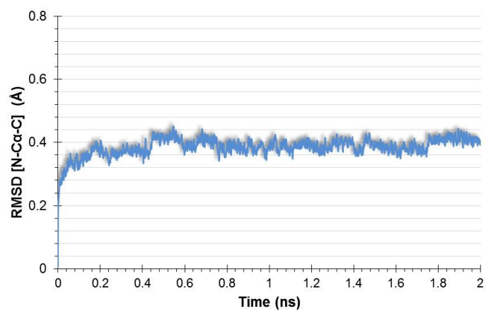
Figure S1. Time-dependent evolution of the RMSD of the protein backbone atoms along the 2 ns QM/MM MD simulation of HG-3.
