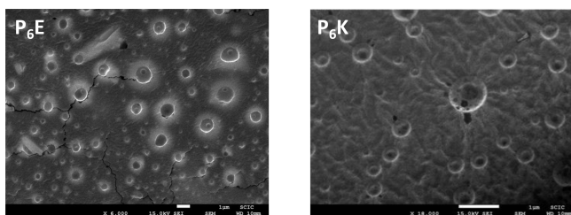
Figure 5. Scanning electron microscopy images of vesicle-like assemblies of \text{P}_6\text{E} and \text{P}_6\text{K} (1% w/w) formed at 80 ^\circ\text{C} in phosphate buffer at pH 7. The sample was fast frozen and lyophilized prior to observation. Scale bars are 1 \mu\text{m} long.
