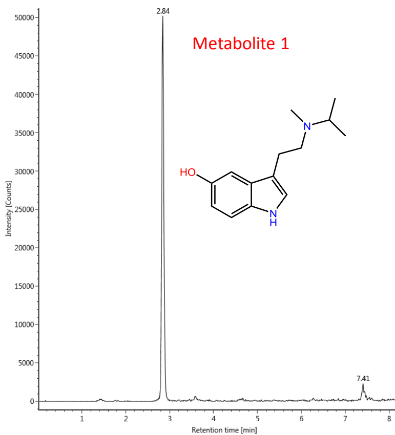
Figure 7. EICs corresponding to the protonated molecule of 5-MeO-MiPT (top) and Metabolite 1 (bottom) in hydrolysed urine, collected 24 hours after administration.
