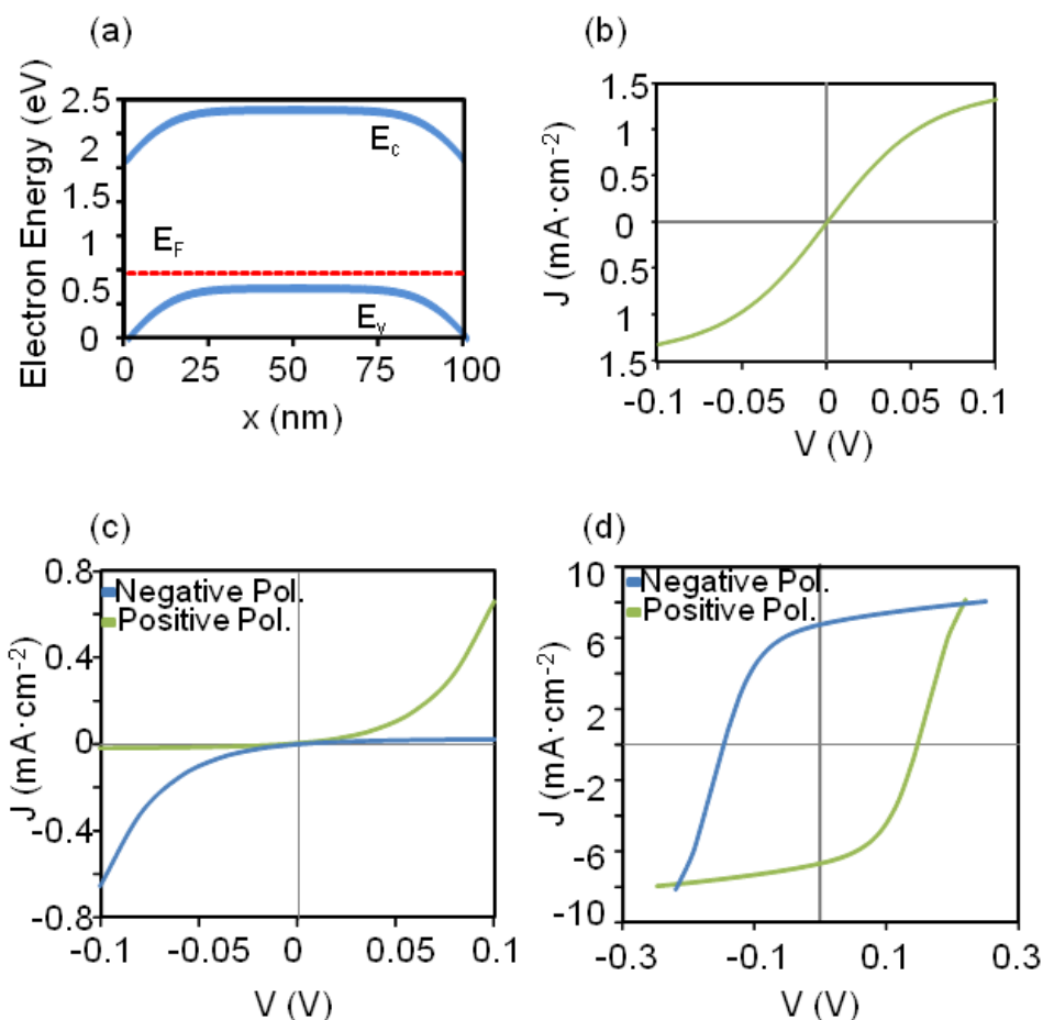
Fig. 25. (a) Electron energy scheme of a symmetric Schottky MFM structure with the following parameters of the ferroelectric semiconductor: doping concentration of N_A=10^{17} \text{ cm}^{-3} , film thickness of d=100 \text{ nm} , \mu = 1 \text{ cm}^2/\text{Vs} and \epsilon_r = 10 . The height of the energy barriers at the contacts are considered to be 0.8 \text{ eV} . (b) Current-voltage characteristic for this MFM structure in dark with no poling effects. The semiconductor is considered ferroelectric (c), (d) Current-voltage characteristics in the MFM structure under positive and negative (c) polarization without and (d) with illumination.
