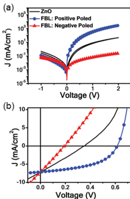
Fig. 32. (a) Electrical characteristics of a device ITO/ferroelectric blend layer(110 nm)/Al under electrical poling. The blend layer is a mixture of ZnO and P(VDF-TrFE). (b) Current density-voltage curves of bulk heterojunction organic solar cell, with a ferroelectric blend layer, at one sun illumination intensity. Reprinted from (Jo et al., 2015).
