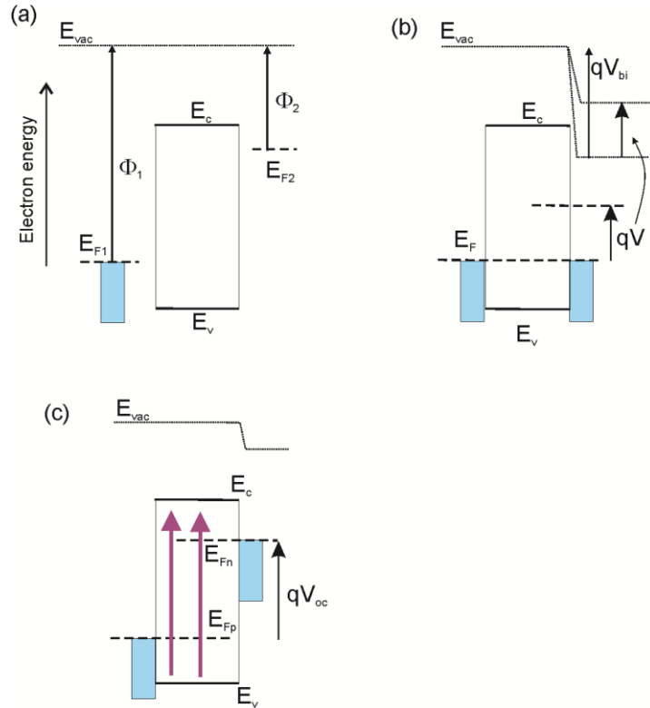
Fig. 3. Formation of an elemental diode-like device. (a) Separate materials, a semiconductor with conduction band edge minimum E_c and valence band maximum E_v , and two contacts with work function \Phi_1 and \Phi_2 . (b) Equilibration of Fermi levels for the materials in contact, by formation of a surface dipole indicated in the vacuum level (VL). The situation of an applied voltage V is also shown. (c) Under photogeneration, the diode is a solar cell that produces a photovoltage.
