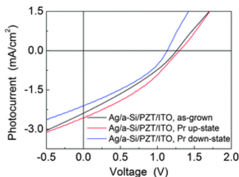
Fig. 16 (a) J - V measurements at 2.85 suns of ITO/BFO(>200 nm)/SRO (Yang et al., 2009) (b) J - V characteristics of Ag/a-Si/PZT/ITO/glass samples illuminated under simulated standard sunlight (AM 1.5, 100 \text{ mW cm}^{-2} ) when the PZT films were in the as-grown state (no poling voltage), remnant polarization pointing to the top electrode (up-state, +10 V poling for 5 s), and remnant polarization pointing to the bottom ITO electrode (down-state, -10 V poling for 5 s), respectively. Here, the reference voltage was defined as a positive voltage applied on the bottom ITO electrode. Reproduced from (Hu et al., 2016).
