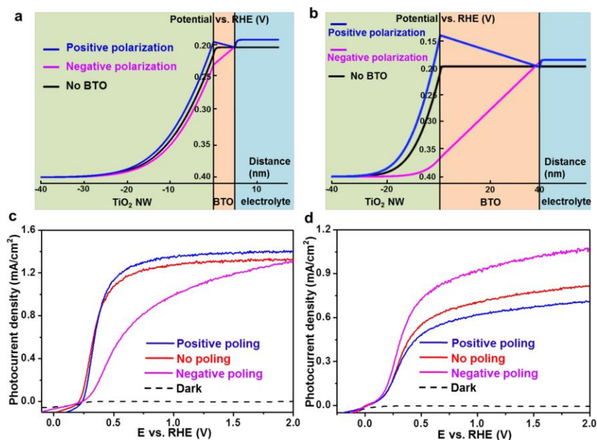
Fig. 34. (a) Calculated potential distribution and electric poling test of the ferroelectric enhancement. (a) Potential distribution of 150 °C \text{TiO}_2/5 nm BTO/NaOH heterojunction, where the spontaneous polarization in BTO shell induced an upward band bending of \text{TiO}_2 core and facilitated the charge separation and transportation inside \text{TiO}_2 . (b) Potential distribution of the 210 °C \text{TiO}_2/40 nm BTO/NaOH heterojunctions,
