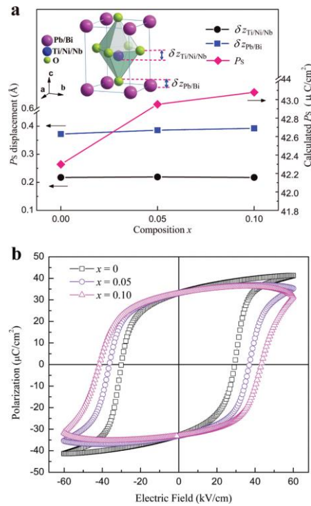
Figure 2. The figure shows a generic behaviour of a ferroelectric oxide perovskite with a general formula \text{ABO}_3 . (a) The displacement and the calculated P_s of 0.65\text{PbTiO}_3 - 0.35\text{Bi}(\text{Ni}_{2/3+x}\text{Nb}_{1/3-x})\text{O}_{3-\delta} as function of x . The inset displays the spontaneous polarization displacement at A and B sites in the perovskite lattice. (b) Hysteresis loops of 0.65\text{PbTiO}_3 - 0.35\text{Bi}(\text{Ni}_{2/3+x}\text{Nb}_{1/3-x})\text{O}_{3-\delta} ( x = 0, 0.05, \text{ and } 0.10 ) ceramics measured at a frequency of 1 Hz. Reprinted from (Liu et al., 2015).
