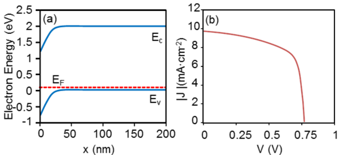
Fig. 6. (a) Band diagram for a Schottky barrier solar cell in the dark. (b) Corresponding current density-voltage characteristic. The parameters used in the numerical simulation are reported in the Table 1 of SI.
