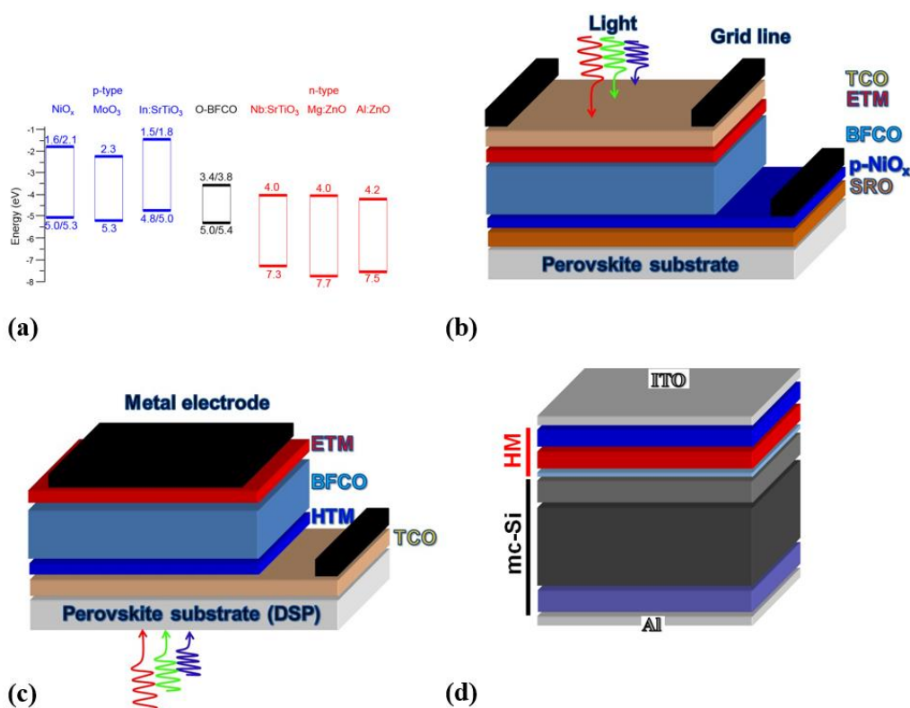
Fig. 37. (a) Schematic descriptions of the energy level diagram of (\text{NiO}, \text{MoO}_3) \text{In-SrTiO}_3/\text{BFCO}/\text{Nb-SrTiO}_3 ( \text{Al:ZnO}, \text{Mg:ZnO} ). Structure of (b) conventional and (c) inverted p - i - n junction types of semiconducting BFCO PV devices. (d) Schematic representation
