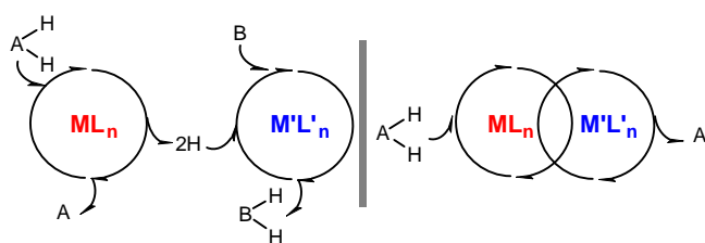
Figure 1. Multimetallic (de)hydrogenation catalysed processes.
