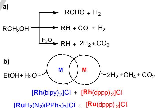
Scheme 2. Alcohol dehydrogenation catalysed by the combination of different metal complexes.
