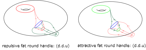
Figure 4: Fat handles associated to operation II of Wada removing a component of h .
