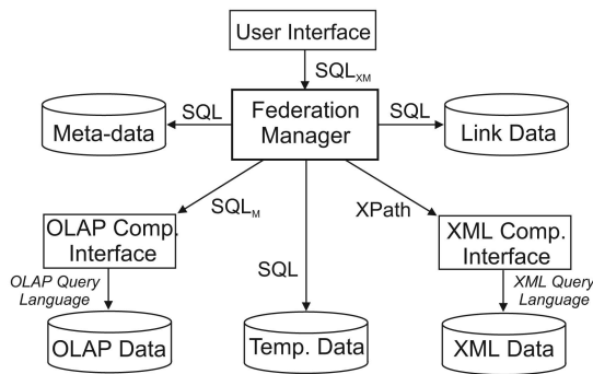
Fig. 11. OLAP-XML federation architecture [19].
