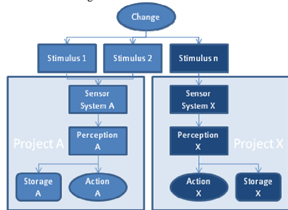
Figure 1: Overview of DENS.
