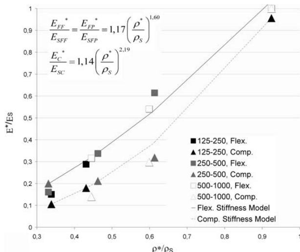
4 Relative stiffness and compression according to relative density (adjusted for developed models)
