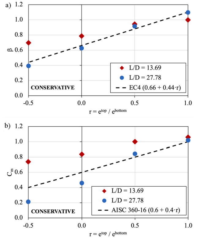
Fig. 11. Equivalent moment factor ( \beta \cdot C_m ). Measured and predicted. a) EC4. b) AISC 360-16.
