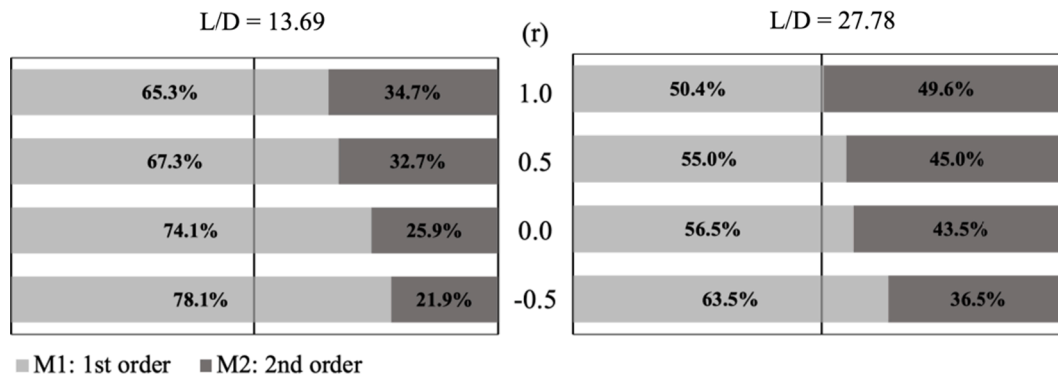
Fig. 12. First and second order bending moment obtained from experiments.
