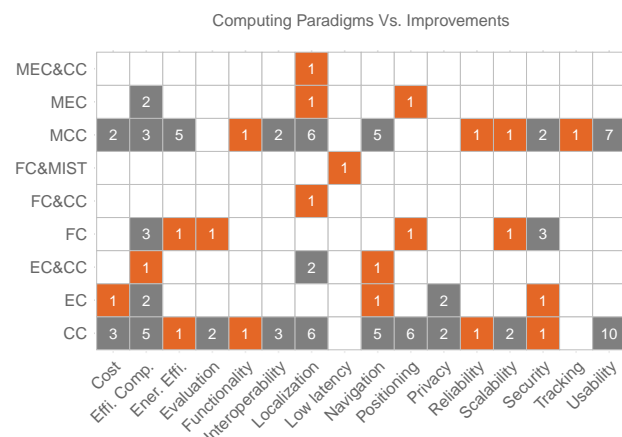
Figure 5. Computing paradigms and studies analysed main goals.
