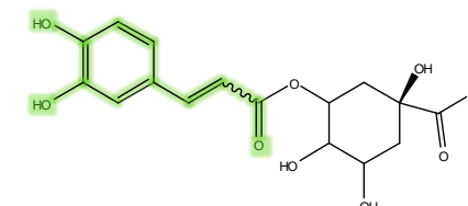
Fragment [C9H7O3-H]-H^- Theoretical m/z 161.0244 Error(mDa) -1.2
