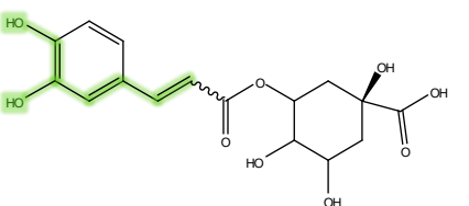
Fragment [C6H5O2+2H]^- Theoretical m/z 111.0452 Error(mDa) -1.85
