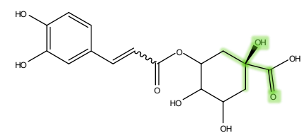
Fragment [C4H5O2]^- Theoretical m/z 85.0295 Error(mDa) -1.7
