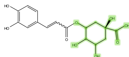
Fragment [C7H11O6]^- Theoretical m/z 191.0561 Error(mDa) -1.2
