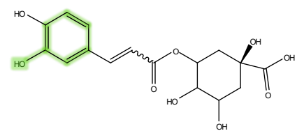
Fragment [C6H4O+H]^- Theoretical m/z 93.0346 Error(mDa) -1.18
