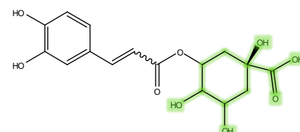
Fragment [C7H11O5-H]-H^- Theoretical m/z 173.0455 Error(mDa) -1.0
