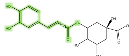
Fragment [C9H7O4]^- Theoretical m/z 179.0350 Error(mDa) -2.0
