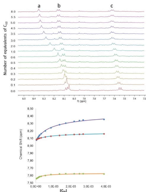
Figure 2. Selected regions of the 1 H NMR (500 MHz, toluene- d 6 , 298 K) spectra acquired during the titration of 5 with incremental amounts of C 60 . The concentration of 5 was maintained constant (0,5 mM) throughout the titration. The binding isotherm is shown below.
