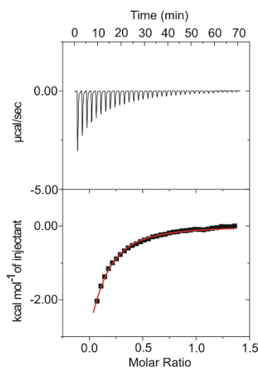
Figure 4. (top) Heat vs time plot of the ITC experiment of 5 (0.6 mM) with incremental additions of C_{60} (3.8 mM), in toluene at 298 K. (bottom) The best fit of the integrated heats to the theoretical binding isotherm obtained assuming three ( N = 3 ) equivalent binding sites in C_{60}@5_3 . The resulting thermodynamic data ( K , \Delta H , and \Delta S ) are per mole of 5 .
