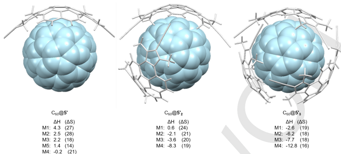
Figure 7. Optimized geometries of C_{60}@5'_n ( n = 1 - 3 ). The enthalpies (kcal/mol) and entropies ( \text{cal}\cdot\text{K}^{-1}\cdot\text{mol}^{-1} ) of formation are in toluene at 298 K, per mole of \text{toluene}_2@5 , calculated with methods M1 – M
