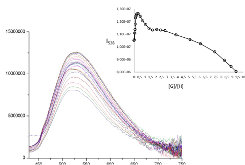
Figure 3. Fluorescence spectra acquired during the titration of 5 ( 1.55 \times 10^{-5} M) with C_{60} ( 2 \times 10^{-3} M) in toluene at 298 K ( \lambda_{\text{exc}} = 403 nm). The inset plot represents \Delta I_{528} against the number of added equivalents of C_{60} .
