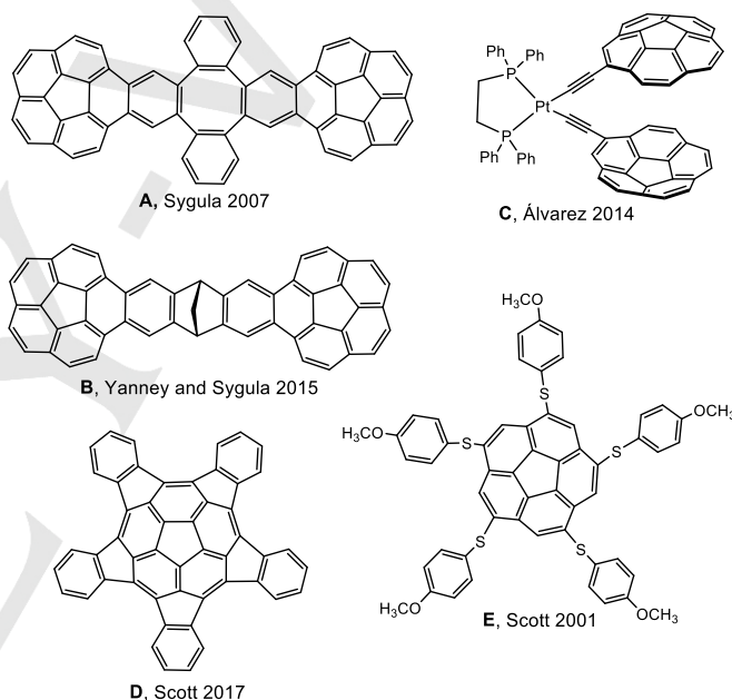
Chart 1. Line-drawing structures of 'buckycatchers' A-C , pentaindecorannulene D , and corannulene derivative E featuring five geodesic electron-rich arms
