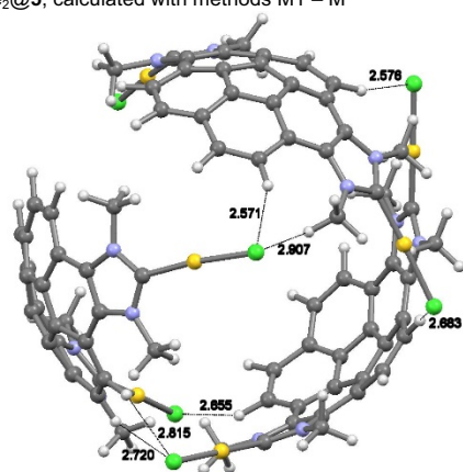
Figure 8. Optimized geometries of C_{60}@5'_3 showing some intermolecular \text{Cl}\cdots\text{H} interactions. C_{60} was removed from the structure for clarity. Distances in Å.
