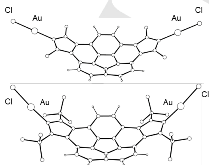
Figure 5. Geometries of 5' (above) and 5 (below) calculated using the \omega B97XD (M5) method.
