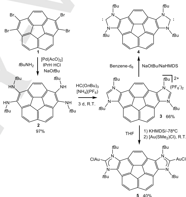
Scheme 1. Synthesis of corannulene derivatives 2-5.
