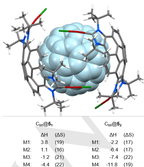
Figure 9. The optimized geometry of C_{60}@5_2 . The enthalpies (kcal/mol) and entropies ( \text{cal}\cdot\text{K}^{-1}\cdot\text{mol}^{-1} ) of formation of C_{60}@5 and C_{60}@5_2 are in toluene at 298 K, per mole of \text{toluene}_2@5 , calculated with methods M1 – M4.
