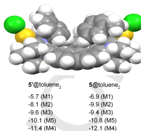
Figure 6. The space-filling view of toluene 2 @ 5 . The enthalpies (kcal) of toluene binding to 5 and 5' are in toluene at 298 K, per mole of toluene, calculated with methods M1 – M5.
