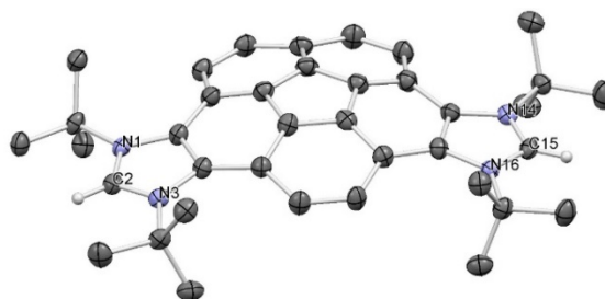
Figure 1. X-ray structure of 3 . Thermal ellipsoids set at 50% probability. Hydrogen atoms (except hydrogens at NCHN), counter-anions ( 2PF_6^- ) and solvent (1,2-dichloroethane) are omitted for clarity. Selected bond distances (Å) and angles ( ^\circ ): N(1)-C(2) 1.319(3), N(3)-C(2) 1.326(3), N(14)-C(15) 1.331(3), N(16)-N(15) 1.323(3), N(1)-C(2)-N(3) 112.0(2) , N(16)-C(15)-N(14) 111.5(2) .
